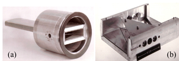
Figure 1: Pictures of an SPS BPH: full BPH assembly (a), and partly dismantled BPH inner body (b).
