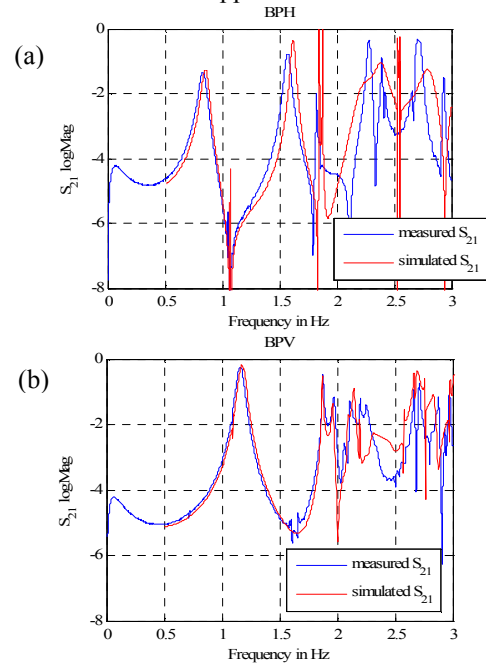
Figure 5: Microwave Studio simulations (red) and RF bench measurements (blue) of the scattering parameter S_{21} for (a) the SPS BPH and (b) the SPS BPV. Contrary to Fig. 4, the ceramics plots behind the electrodes were included in the simulations
