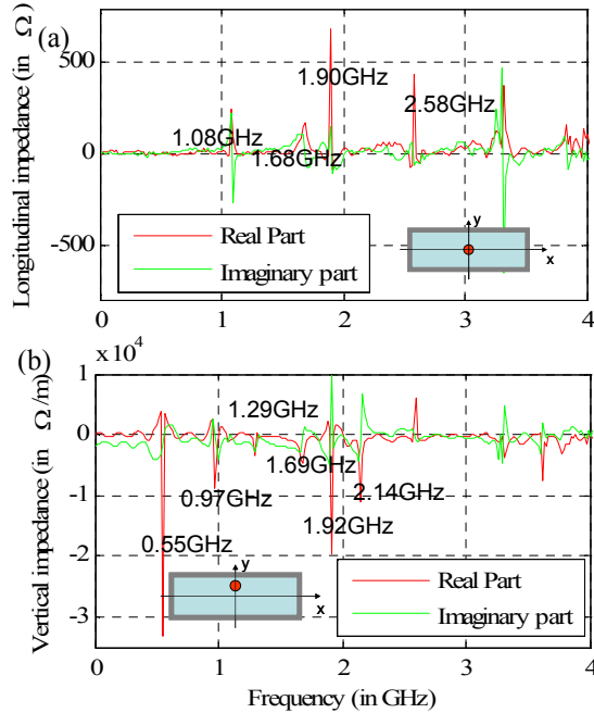
Figure 3: SPS BPH: longitudinal impedance (a) and total (dipolar + quadrupolar contributions) vertical impedance (b) spectra. The main resonance frequencies are displayed by the peaks. The total vertical impedance is normalized to the 5 mm vertical displacement.
