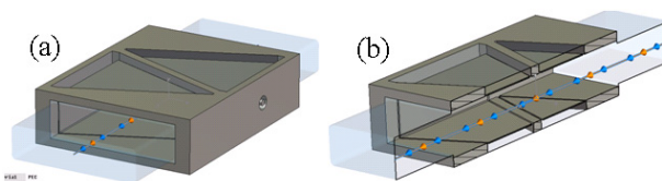
Figure 2: Model of the SPS BPH: (a) Beam path and wake integration path are shown with blue and orange arrows. Using a cut plane (b) reveals the inner structure of the BPH body: a pair of bi-triangular shaped electrodes isolated from the rest of the casing with vacuum cavities. Beam entry and exit planes are perfect matching layers, and all other boundaries are PEC.
