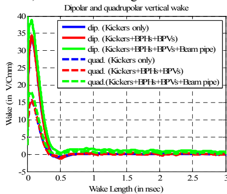
Figure 4: Vertical dipolar and quadrupolar wakes for the summed \beta -weighed contributions of the SPS kickers, the wall impedance of the beam pipe and all BPHs and BPVs.
