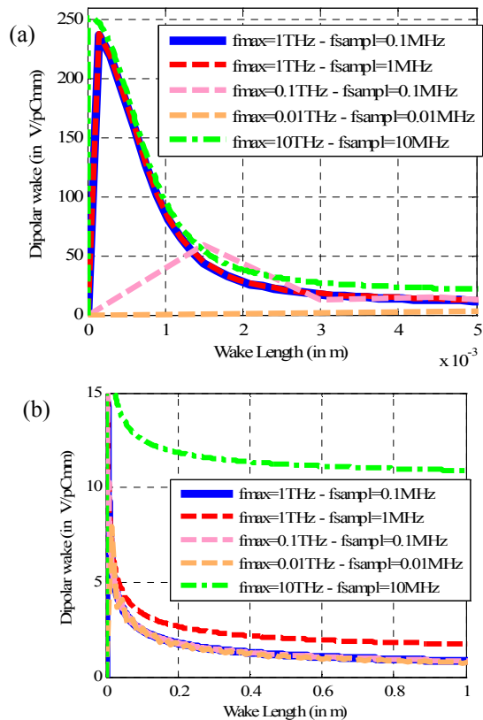
Figure 2: Transverse wake function obtained by DFT of the impedance shown in Fig. 1 up to 5 mm (a), and up to 1 m (b) for different frequency samplings (0.01 MHz to 10 MHz) and frequency span (0.01 THz to 10 THz). The wake obtained from the largest number of impedance points (blue thick line, 0 to 1 THz with a sampling of 0.1 MHz, i.e. 10^7 points) seems to be a fair compromise at both low (a) and high (b) distance to the source charge.
