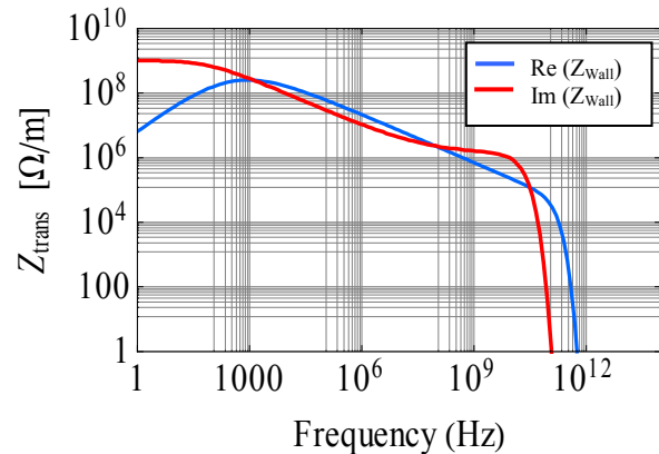
Figure 1: Transverse Wall impedance for a model SPS Beam Pipe (round Stainless Steel pipe, with 2 cm radius and 6911 m length, relativistic gamma \gamma = 27.7 ). The wall impedance formula contains both the resistive wall and the perfect conductor wall - also called indirect space charge - contributions of the impedance [10].
