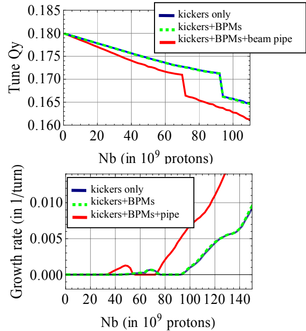
Figure 5: Vertical tune shifts and growth rates obtained from Headtail simulations with Fig. 4 wake functions as inputs.
