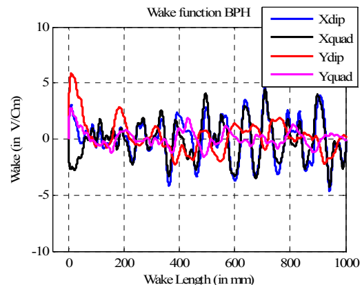
Figure 3: Transverse wake functions for an SPS BPH obtained from CST Particle Studio simulated wake potentials. Linear dipolar and quadrupolar contributions are obtained for each plane by displacing both source bunch and wake calculation transverse locations as explained in Table 2.
