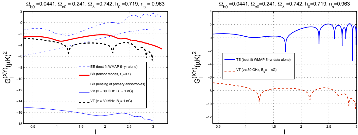
Figure 2: The V-mode power spectra are compared with the linear polarizations. As in Fig. 1 on both axes the common logarithm of the indicated quantity is reported.
