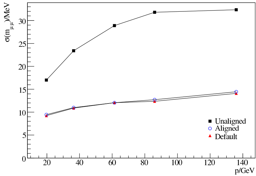
Figure 3. The di-muon mass resolution as function of momentum for default, mis-aligned and aligned scenarios.
