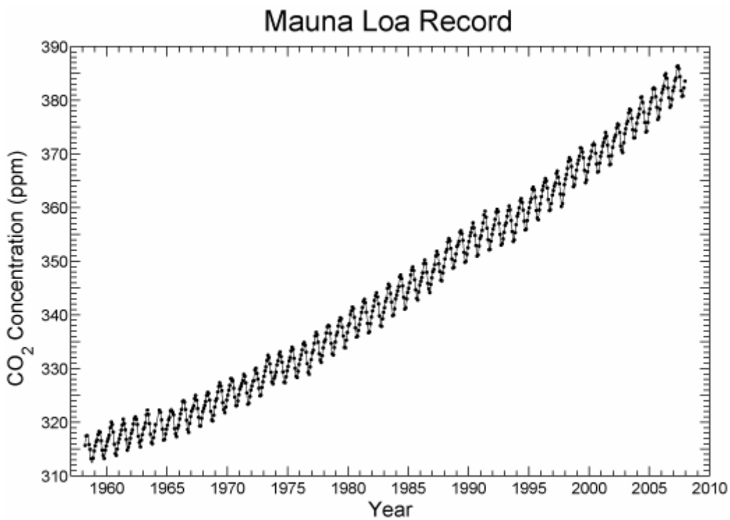
Figure 4: The Keeling Curve 15
