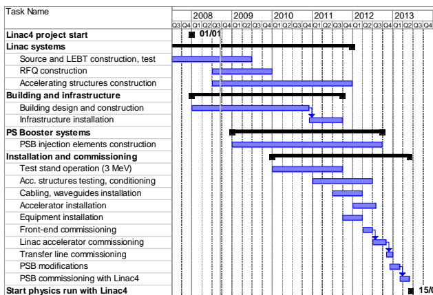
Figure 7: Linac4 Masterplan.
