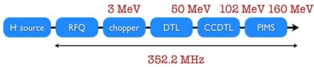
Figure 4: Linac4 layout.
