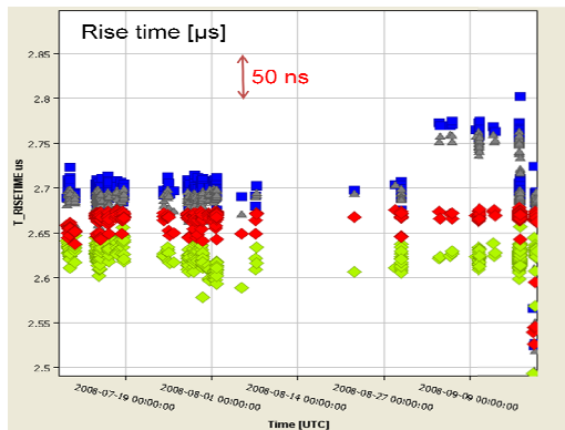
Figure 3: Measured dump kicker rise time at 450 GeV beam energy for four extraction kicker magnets, measured over several months.
