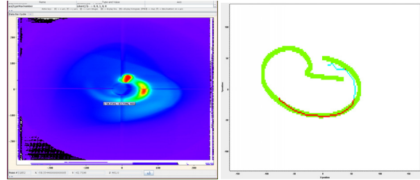
Figure 4: BTVDD image at the left and its XPOC analysis on the right.
