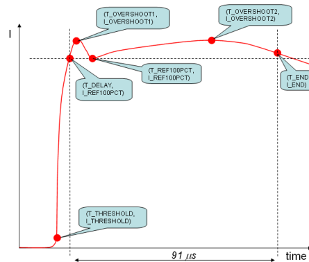
Figure 1: Description of the characteristic points of the extraction kicker current waveform.
