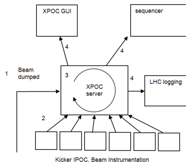
Figure 2: Description of the XPOC system.
