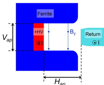
Figure 1: Simplified cross-section of a kicker magnet.
