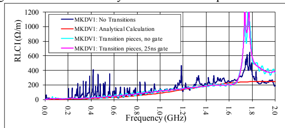
Figure 7: RLCI for MKDV1.
