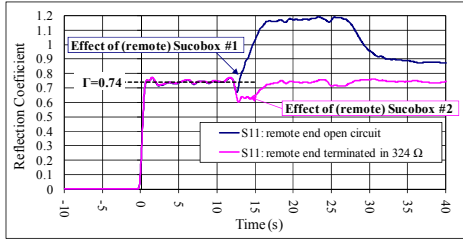
Figure 4: S 11 measurement for the MKDH3 kicker.
