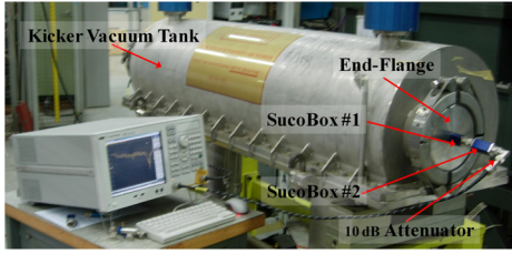
Figure 3: Longitudinal impedance measurement setup.
