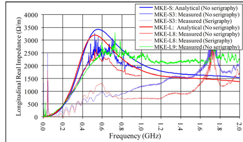
Figure 6: Measured and theoretical RLCI for MKEs.
