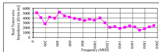
Figure 8: Real TDHI for MKDH3.
