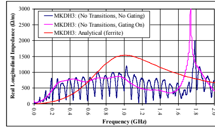
Figure 5: Measured and theoretical RLCI for MKDH3.
