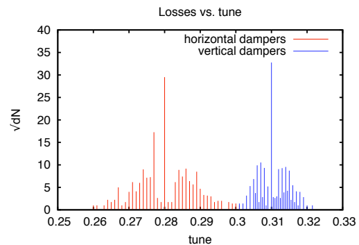
Figure 5: Number (sqrt) of lost particles vs. excitation frequency
