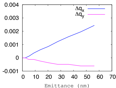
Figure 6: Tune variation vs. particle emittance (by FFT of Turn-By-Turn data, luminosity optics with errors).
