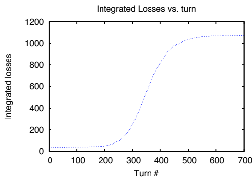
Figure 2: Integrated losses vs. turn number for the injection case with reduced vertical kick.
