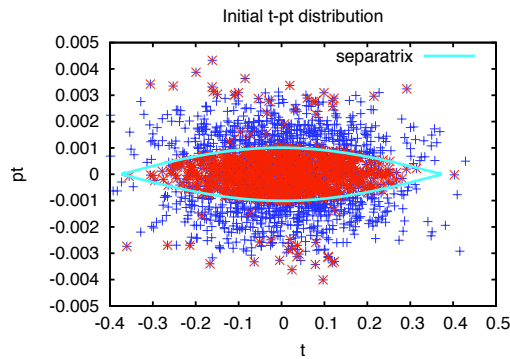
Figure 1: Initial longitudinal particle distribution for the injection energy case; in red are particles which will be lost when kicking at the nominal vertical betatron frequency and maximum kick reduced by a factor 10 together with the separatrix (cyan).
