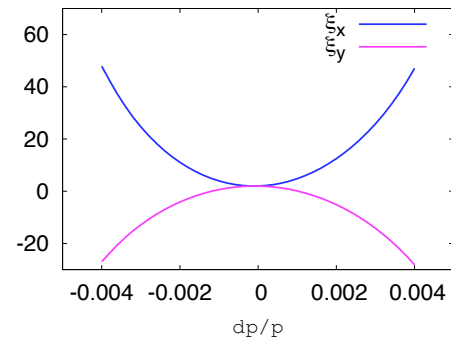
Figure 4: Chromaticities vs. momentum (MAD-X, injection optics with errors).
