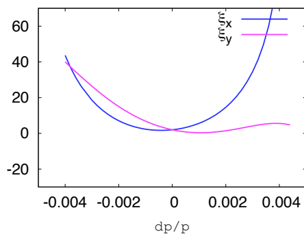
Figure 7: Chromaticities vs. momentum error (MAD-X, luminosity optics with errors).
