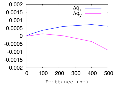
Figure 3: Tune variation vs. particle emittance (by FFT of Turn-By-Turn data, injection optics with errors).
