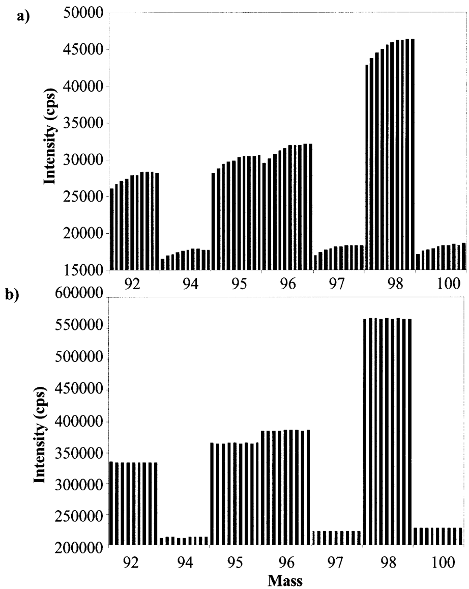
Figure 2.2 Comparison of Mo standards run before (a) and after (b) manual Mo mass calibration or mass offset correction.
