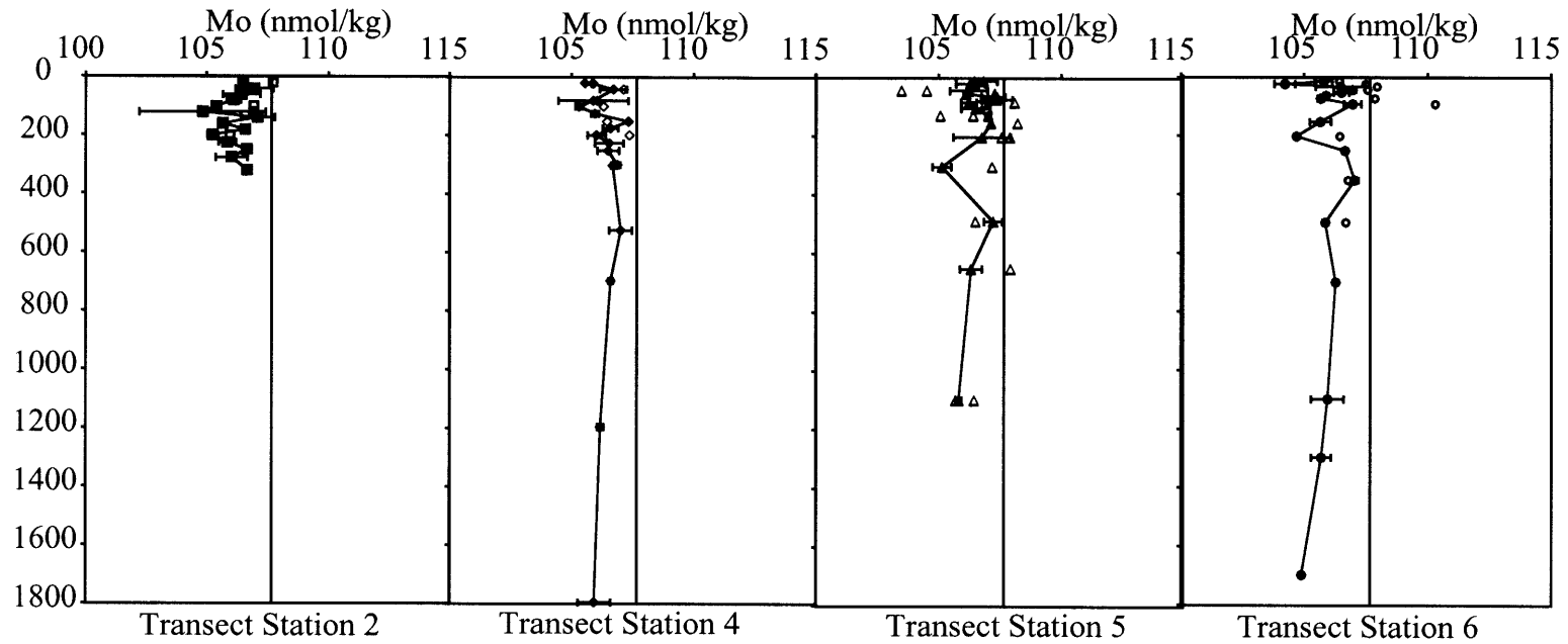
Figure 3.9 Mo profiles of unfiltered niskin samples (open symbols) and filtered niskin samples (closed symbols) from a transect from Hawaii to the coast of Mexico collected in 2000 by Eric DeCarlo. Molybdenum concentrations are salinity normalized to 35ppt. Error bars on Mo indicate average replicate precision. The straight line at 107.67 nmol/kg represents the nominal conservative value of Mo.
