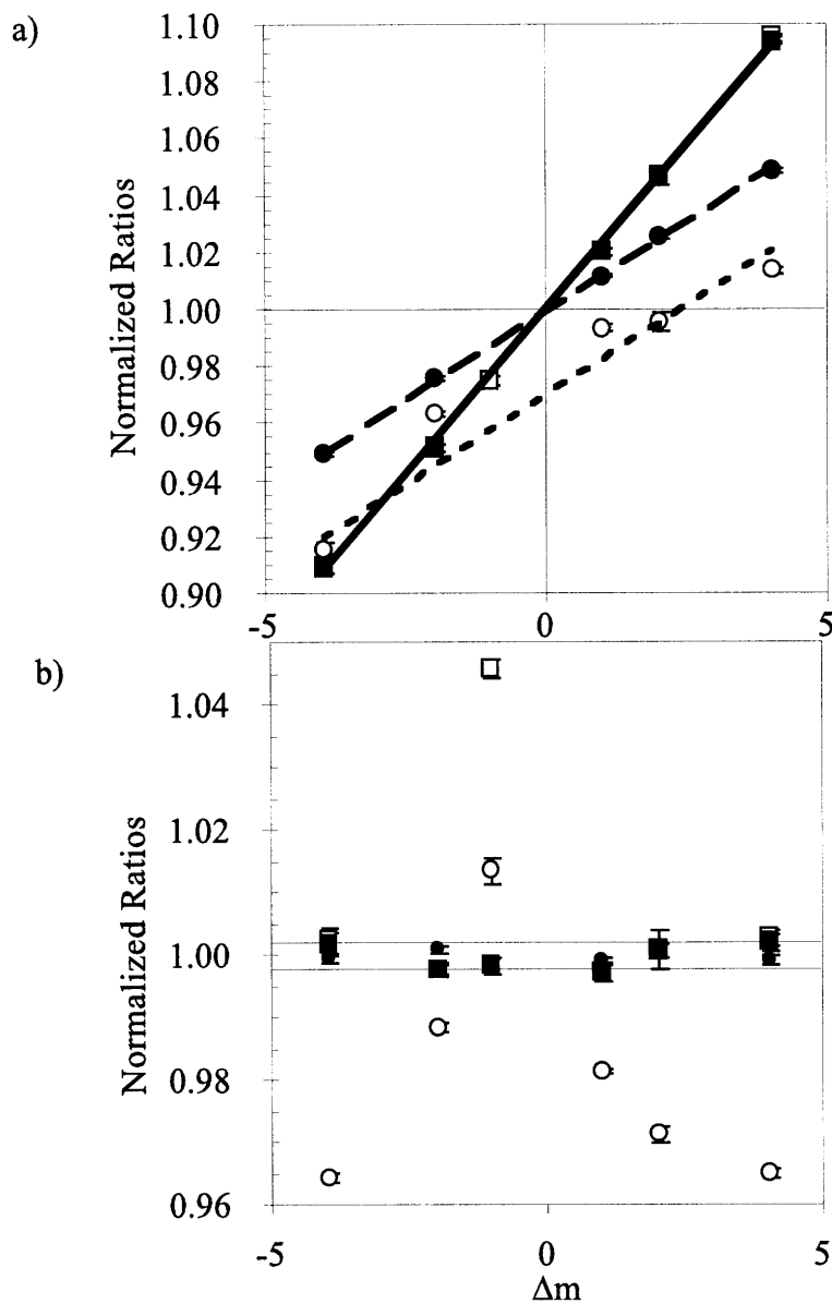
Figure 2.9 a) Plot of R_m/R_t versus \Delta m of the unspiked masses for a standard (open squares) and a sample solution (open circles). The spiked sample has a poor correlation coefficient and a depressed intercept. This is due to the small contributions of non-spike masses in the spike. To correct for this spike contribution, the R_m of 95/96 is projected onto the spike sample mixing line for each ratio and the true isotopic ratio for the mixture is determined called R_p , projected (Figure 2.3). The solid symbols show R_m/R_p plotted versus \Delta m of the unspiked masses for the same standard and a sample solution as the open symbols. Both sample and standard show better correlation and a n intercept closer to 1. b) Plot of mass bias corrected normalized ratios for samples and standard shown in (a) demonstrates that using R_p rather than R_t normalized ratios to determine fractionation coefficient improves the precision of the mass bias correction. All corrected isotopes fall within \pm 0.2\% of normal values.
