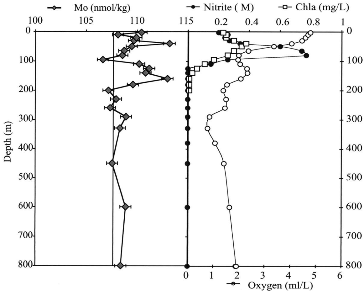
Figure 3.3 Galapagos station 1S 95W profiles of unfiltered niskin samples for Molybdenum (grey diamonds) Nitrite (filled circles) Oxygen (open circles) and fluorescence (open squares) collected in 1992. Molybdenum concentrations were normalized to a salinity of 35 ppt. The straight line at 107.6 nmol/kg represents the nominal salinity normalized Mo concentration from Collier (1985). This same line is shown for reference in all subsequent Mo concentration profiles. Error bars on Mo are -0.5\% . Mo concentrations are enriched in surface waters but approaches conservative values at depth.
