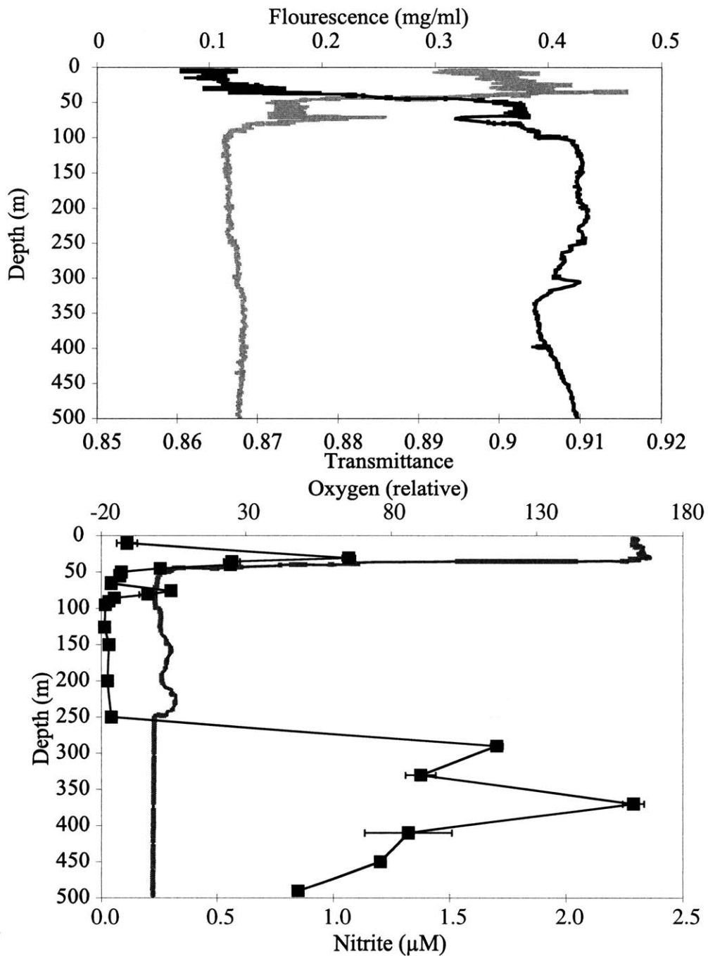
Figure 5.3 Profiles of fluorescence (light gray line), transmittance (black line), nitrite (black squares), and oxygen dark gray line) from the Eastern Equatorial Pacific site 9^{\circ}50'N , 104^{\circ}18'W . Oxygen values are only relative concentrations due to a faulty oxygen sensor. Notice the split shallow nitrite and fluorescence peaks at the top and within the shallow oxygen minimum.
