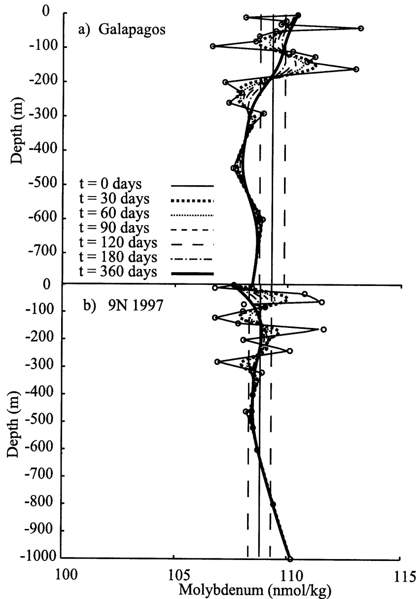
Figure 3.17 Model results from a simple one dimension vertical advection diffusion model used to determine the life time of Mo concentration anomalies in the absence of Mo fluxes. 1 Profiles from the Galapagos (a) and 9N 1997 (b) used as examples. The profiles were allowed to diffuse from initial measured conditions represented by the circles for a total of 360 days. The model equation was dC/dt = D_v(d^2C/d^2z) + v_v(dC/dz) , where D_v , the vertical diffusion rate, was 1 \text{ cm}^2 \text{ s}^{-1} and v_v , the vertical advection rate, was 0.23 \text{ } \mu\text{m} \text{ s}^{-1} . Diffusion profiles plotted for initial conditions (thin solid line) 30 days (thick dotted line) 60 days (thin dotted line) 90 days (small dash line) 120 days (large dash line) 180 days (dot-dash line) and 360 days (thick line). The straight solid line represents the average concentrations of the profile and the straight dashed lines are the 1 sd error bars ( \pm 0.5 \text{ nmol/kg} ).
