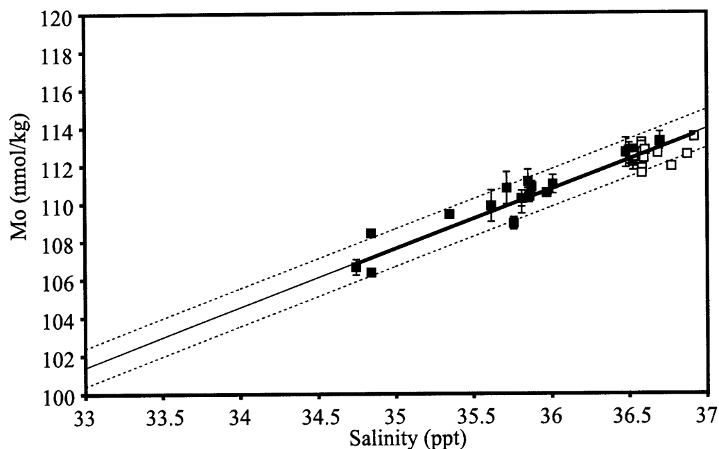
Figure 3.14 Molybdenum versus Salinity diagram for the Arabian Sea (filled squares) and Sargasso Sea (open squares) profiles. Note smaller range in axes than figure 3.9. Error bars from replicate analyses. The solid line is the Mo versus salinity trend measured at lower salinities in the Baltic Sea (Prange and Kremling 1985: \text{Mo nmol/kg} = 3.13 \cdot \text{salinity ppt} - 1.88 ). Dotted lines indicate the average 2 sd error bars ( \pm 1 \text{ nmol/kg} ). Any analysis within 2 sd of the line is considered to be conservative. The thick line is the regression through the Arabian and Sargasso Sea data set. This line is within error of the Baltic Sea trend ( \text{Mo nmol kg}^{-1} = 3.12 \cdot \text{salinity ppt} - 1.80 ). The r-squared correlation coefficient was 0.86. This tight correlation of Mo concentration with salinity indicates that these profiles are conservative.
