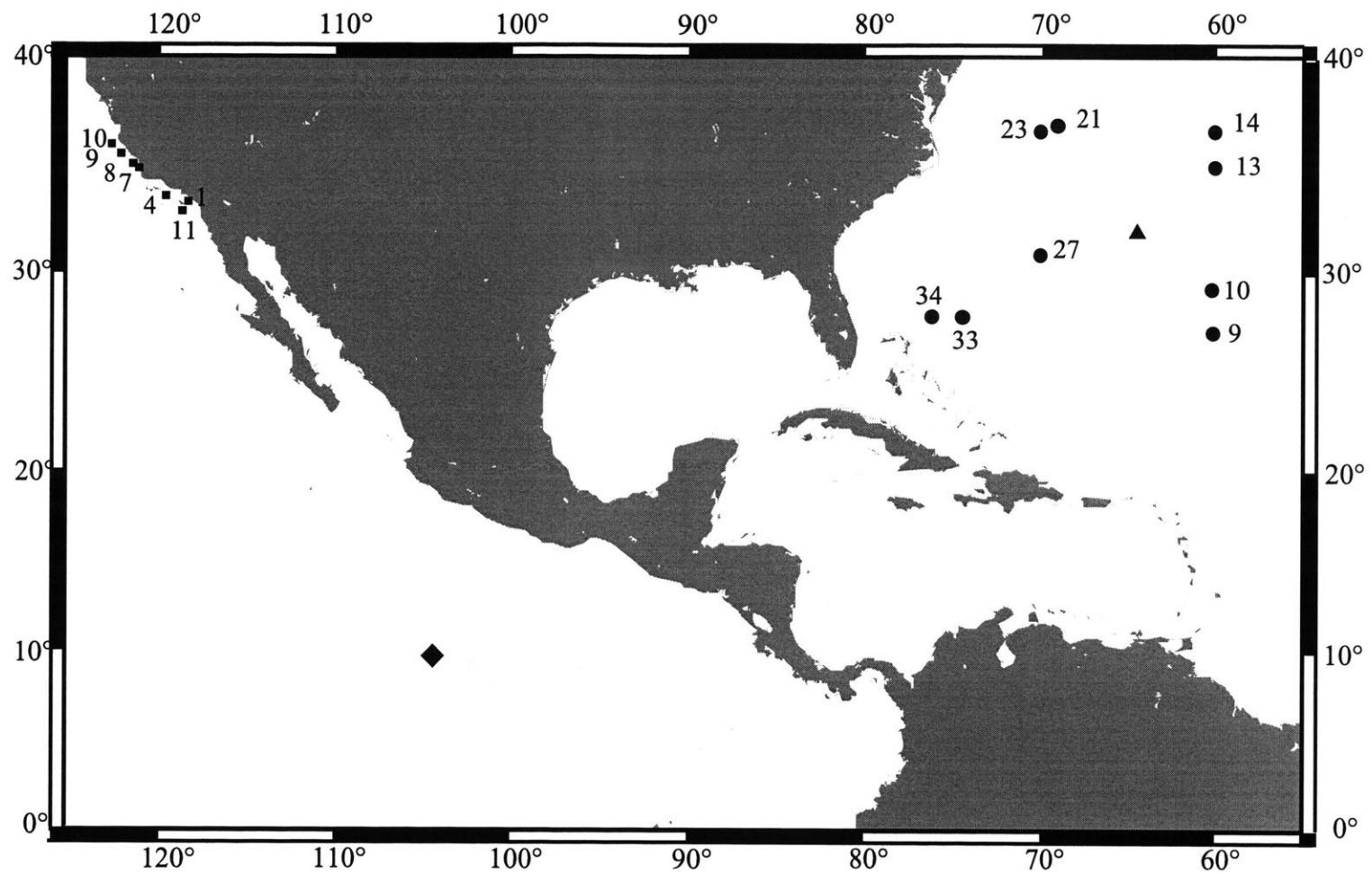
Figure 5.1 Station Location map for SPM samples listed in Table 5.2 including the California Borderland Basin (squares), the 9°N Pacific profile (diamond), the BATS profile (triangle) and the Sargasso Sea Surface Samples (circles)
