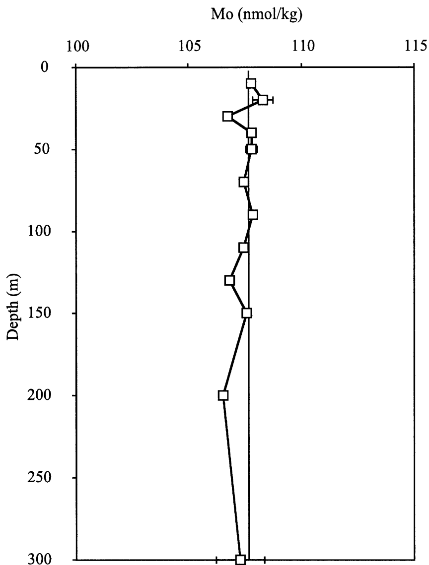
Figure 3.5 Profile of filtered go-flo samples for Mo (open squares) from the Sargasso Sea 25°60N 70°04W collected in 1998. Molybdenum concentrations are normalized to a salinity of 35 ppt. The straight line at 107.6 nmol/kg represents the conservative value of Mo. Error bars on Mo indicate average replicate precision. Mo concentration averaged 107.6 \pm 0.6 (2se) nmol/kg. Concentrations appeared conservative throughout the profile despite low nitrogen concentrations and the presence of nitrogen fixing cyanobacteria.
