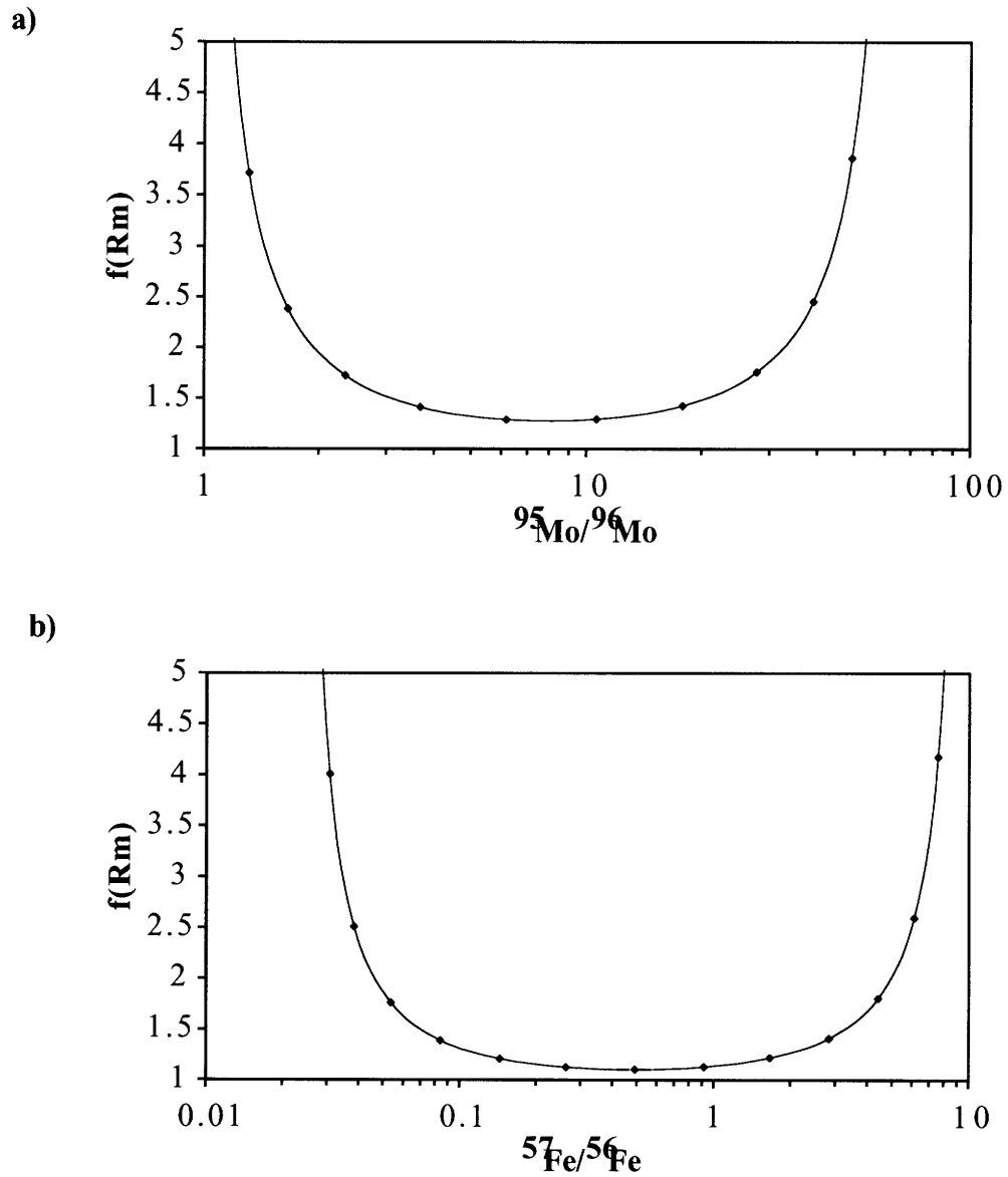
Figure 2.6 Plots f(R_m) versus the N_{sm}/N_{spk} ratio. The minimum represents the optimal range in R_m for a) Mo (6 to 10) and b) Fe (1.6 to 0.14).
