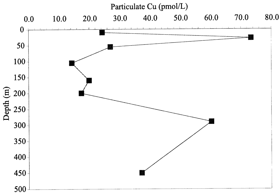
Figure 5.12 Particulate Cu profiles from the Eastern tropical Pacific, 9 50N 104 18W.
