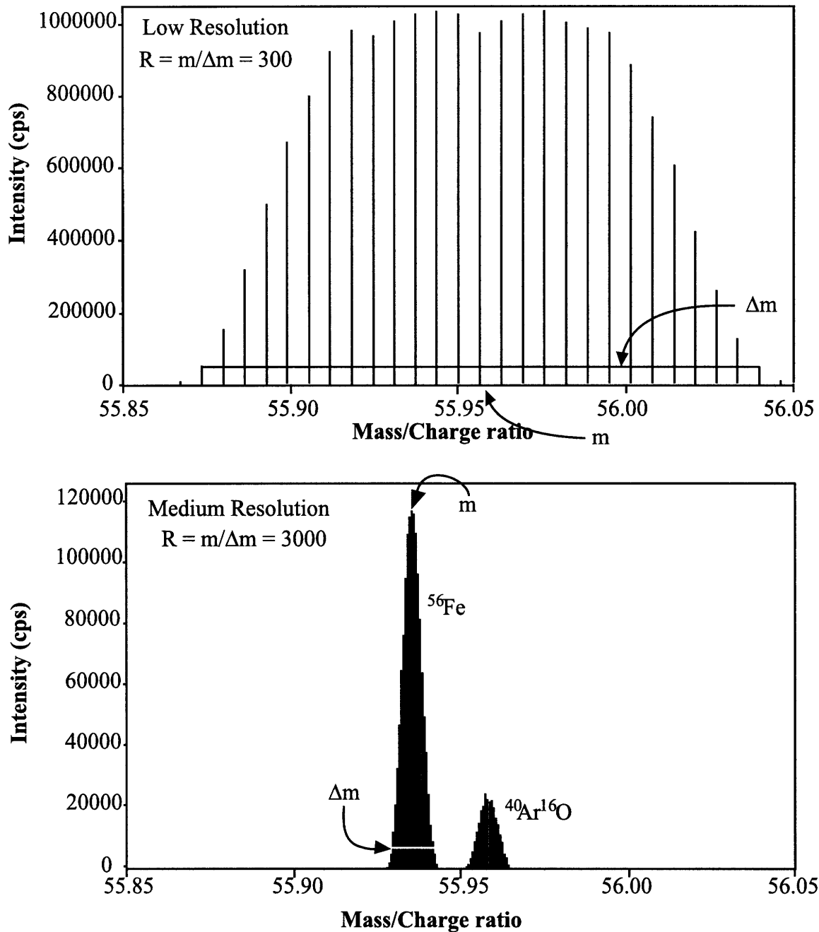
Figure 2.3 Comparison of ^{56}\text{Fe} and ^{40}\text{Ar}^{16}\text{O} peaks as measured in a 1 ppb Fe standard solution with Low (a) and Medium (b) resolution. Resolution ( R ) is defined as the center mass of the peak ( m ) divided by the width of the peak at 5% of the maximum peak height ( \Delta m ). ^{56}\text{Fe} and ^{40}\text{Ar}^{16}\text{O} peaks that are unresolved in low resolution can be easily distinguished with medium resolution. Notice the approximately 12-fold drop in ^{56}\text{Fe} intensity with increasing resolution
