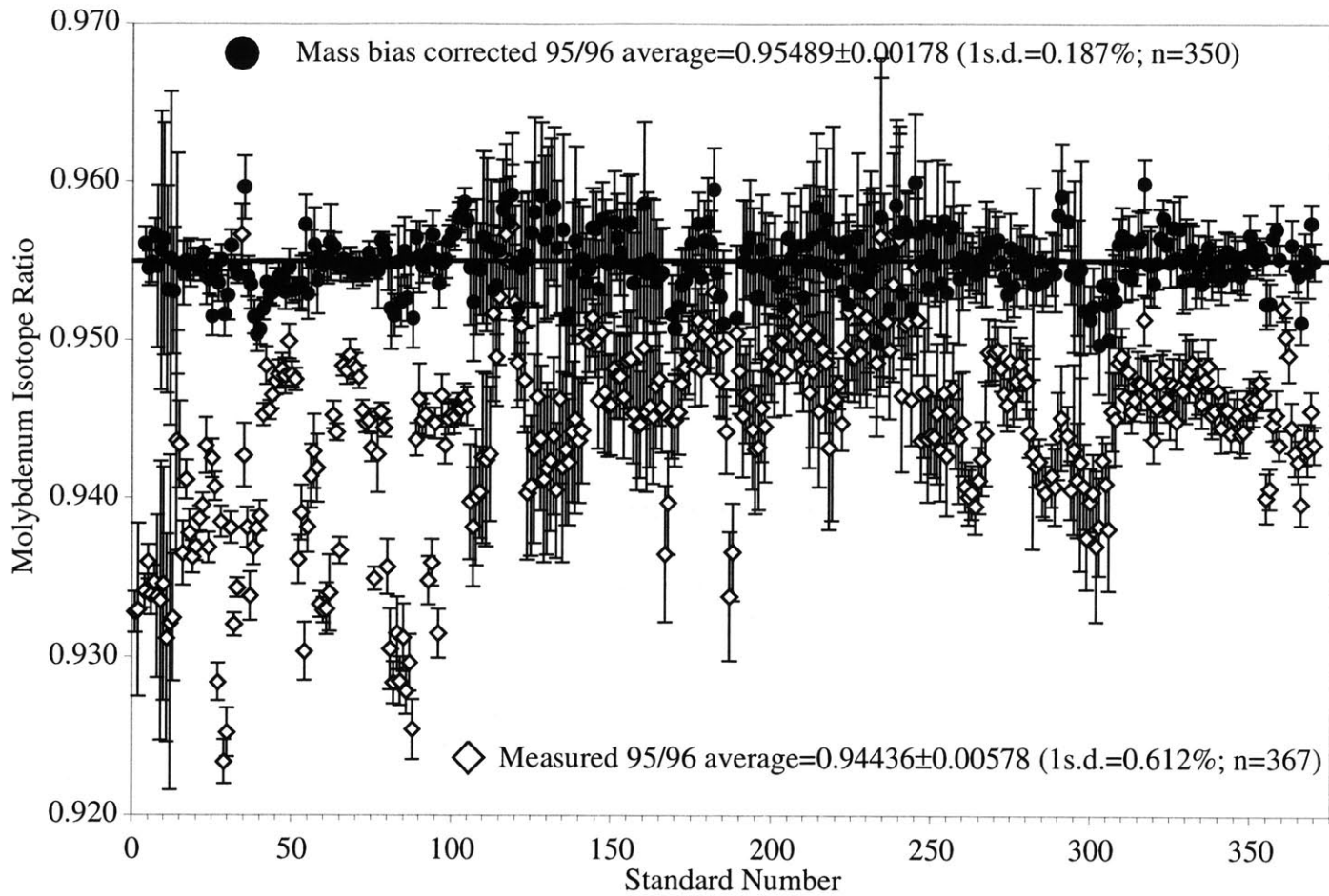
Figure 2.10 Plot of 95/96 Mo ratios from over 350 standard analyses run over the course of 3 years on the WHOI magnetic sector ICPMS. Open diamonds show measured, interference corrected ratios. Filled circles indicate mass bias corrected ratios. The thick black line is the accepted value of 0.955022 (Lee and Halliday 1995) All error bars are one standard deviation measurement errors. The average mass bias corrected ratio is 0.9549 \pm 0.0018 (1SD = 0.19%).
