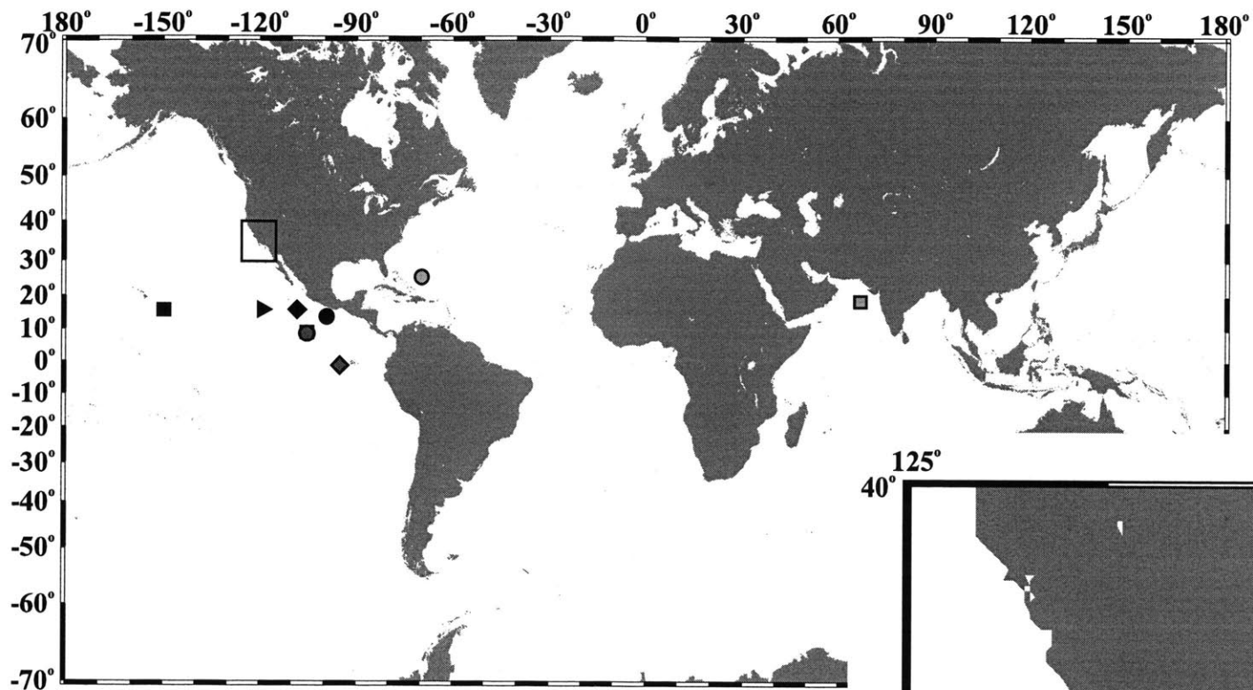
Figure 3.2 A map of station locations including the Arabian (light gray square) and Sargasso Sea (light grey circle) stations, the Eastern Tropical Pacific 16N transect stations 2 (black square), 4 (black triangle), 5 (black diamond) and 6 (black circle), the Galapagos profile (dark gray diamond) and two profiles from 9N collected in 1997 (dark gray square) and 2001 (dark grey circle). Expanded area shows indicated by square shows California Borderland Basin region including profiles from Tanner (open circle), Santa Barbara (open triangle), San Nicholas (open diamond) and San Pedro (open square) Basins.
