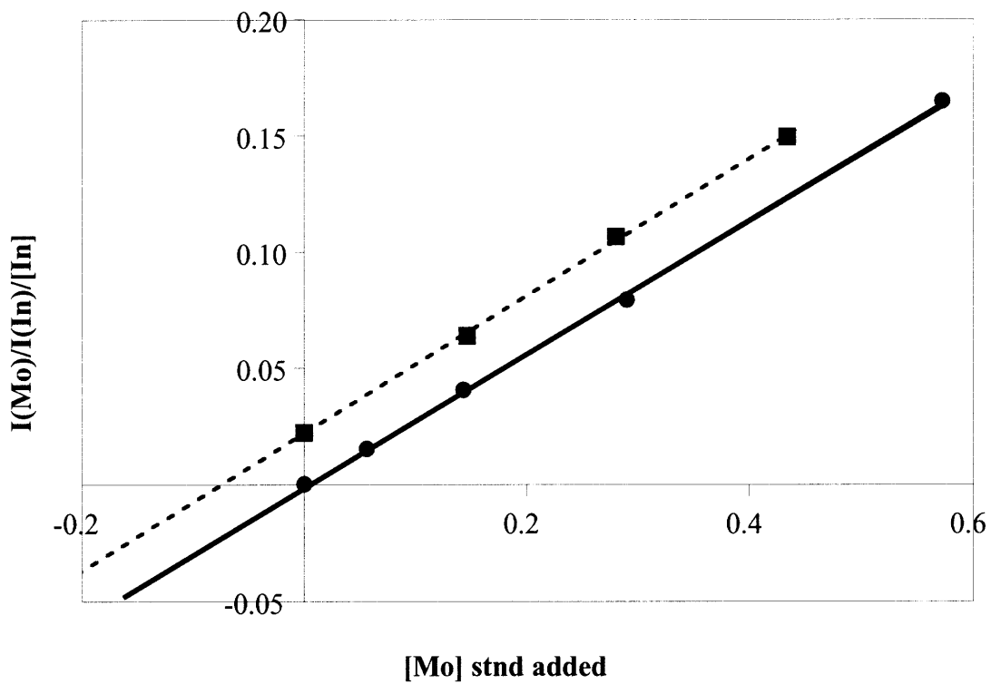
Figure 2.8. Example of Standard Addition lines for a sample (squares) and a standard curve (circles). Slopes are 0.295 and 0.287 for sample and standard, respectively, with intercepts of 0.0219 and 0.0008. The r^2 for each line is 0.999.
