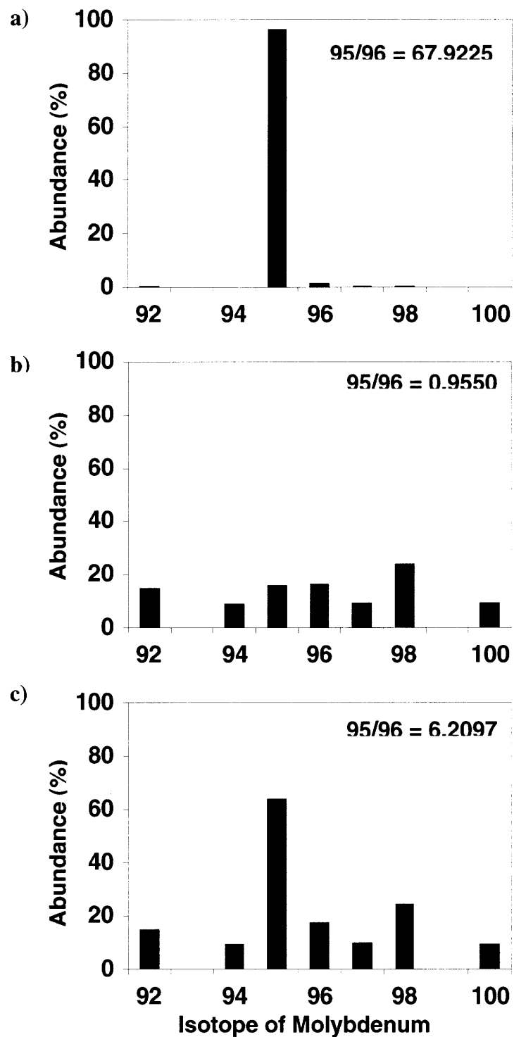
Figure 2.4 Histogram of spike (a) and natural (b) isotope abundances and a mixture (c) of 50% each with calculated 95/96 Mo isotope ratios.
