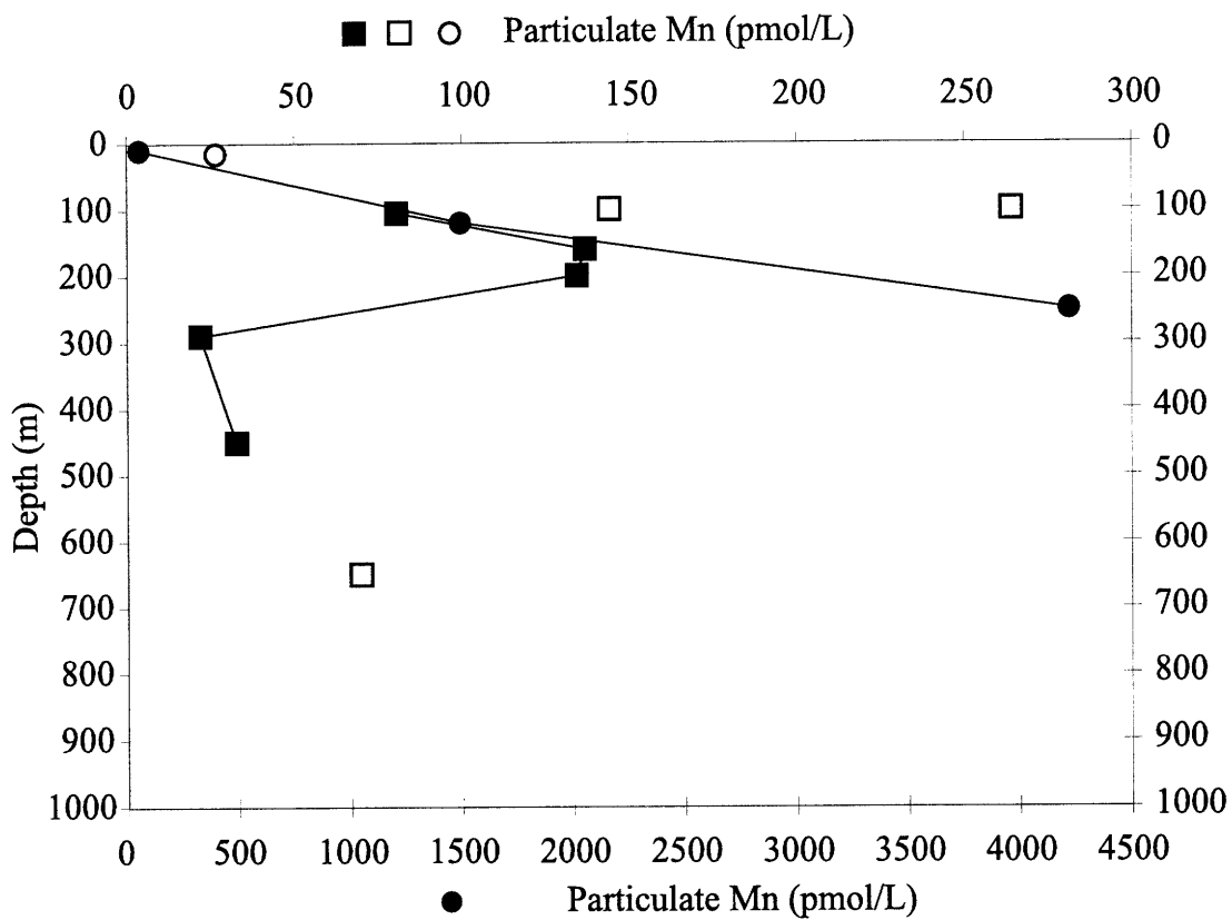
Figure 5.11 Particulate Mn samples from the Eastern Tropical Pacific profile (black squares), BATS profile (black circles), California Borderland Basin samples (open squares) and the Sargasso Sea surface samples (open circles)
