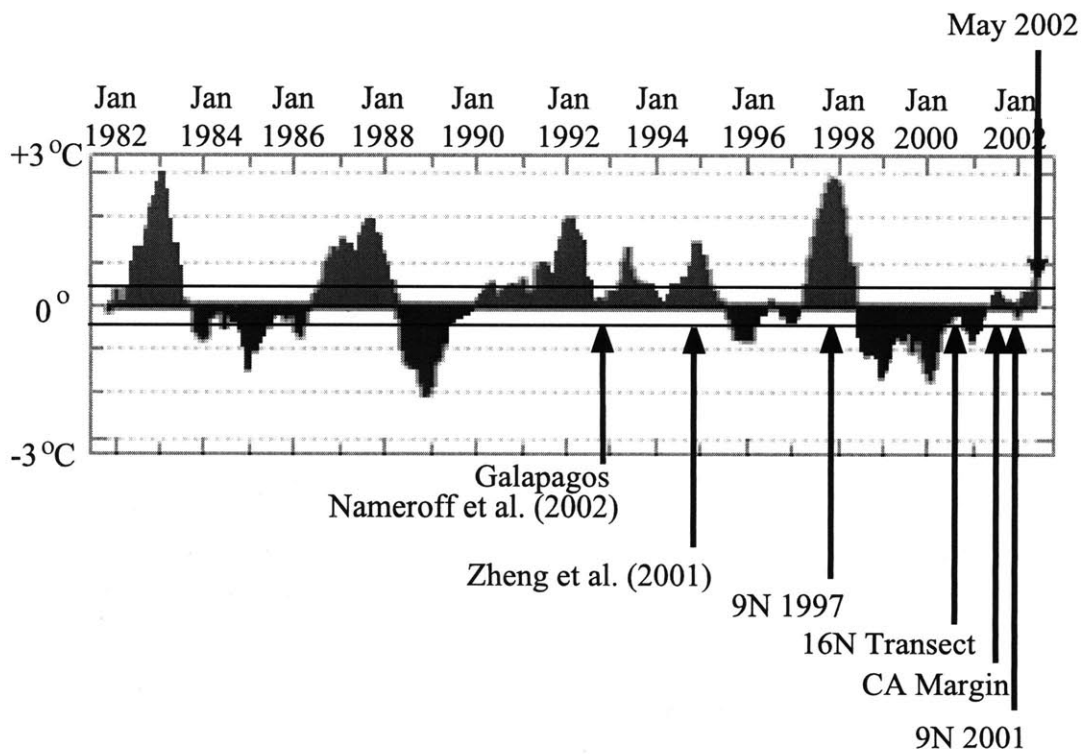
Figure 3.18 Historic Equatorial Pacific sea surface temperature graph for the last 2 decades. Horizontal black lines indicate the normal range in temperature. Peaks above the line indicate El Niño conditions, below the line La Niña conditions. Collection times of Pacific profiles are indicated with arrows. Profiles depleted for Mo were collected during normal to La Niña conditions. Profiles enriched in Mo were collected during or soon after El Niño conditions.
