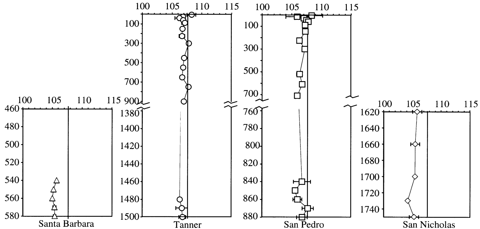
Figure 3.11 Profiles of filtered niskin samples for Mo from 4 California Borderland Basins, Santa Barbara (triangles), Tanner (circles), San Pedro (squares) and San Nicholas (diamonds) collected in 2001. Molybdenum concentrations are salinity normalized to 35ppt. Error bars on Mo indicate average replicate precision. The straight line at 107.6 nmol/kg represents the conservative value of Mo. Profiles focus on the bottom 120m of each basin. Upper water column samples were available for Tanner and San Pedro (note break in scale).
