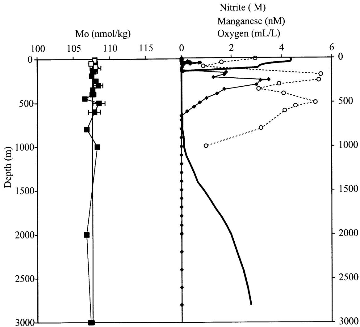
Figure 3.4 Profiles of unfiltered Niskin samples for Mo (black squares), filtered Go-Flo samples for Mo (open squares), Nitrite (black diamonds) Oxygen (thick line) and Manganese (open circles) from the Arabian Sea JGOFS N7 station 19°10N 67°10W collected in 1995. Molybdenum concentrations are normalized to a salinity of 35 ppt. The straight line at 107.6 nmol/kg represents the nominal conservative value of Mo. Error bars on Mo represent average replicate precision. Mo concentration averaged 107.8±0.6 nmol/ kg 2se. Concentrations appeared conservative throughout the profile. Go-Flo and niskin samples agree within error suggesting the Mo can be collected without contamination using a niskin rosette.
