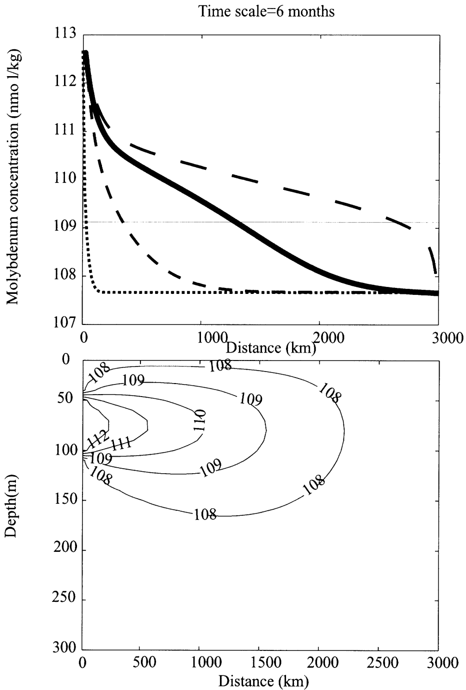
Figure 3.19 Plot of results for 2 dimension forward time center step advection diffusion model used to determine whether Mo concentration anomalies could be advected off shore. A) Plot of concentration at 50m depth for case 1 (thin dotted line: D_h = 106 \text{ cm}^2 \text{ s}^{-1} , v_h = 0 \text{ cm s}^{-1} ) case 2 (small dashed line: D_h = 108 \text{ cm}^2 \text{ s}^{-1} , v_h = 0 \text{ cm s}^{-1} ) case 3 (thick line: D_h = 108 \text{ cm}^2 \text{ s}^{-1} , v_h = 10 \text{ cm s}^{-1} ) case 4 (large dashed line: D_h = 106 \text{ cm}^2 \text{ s}^{-1} , v_h = 20 \text{ cm s}^{-1} ) B) Contour plot of Mo concentration for case3.
