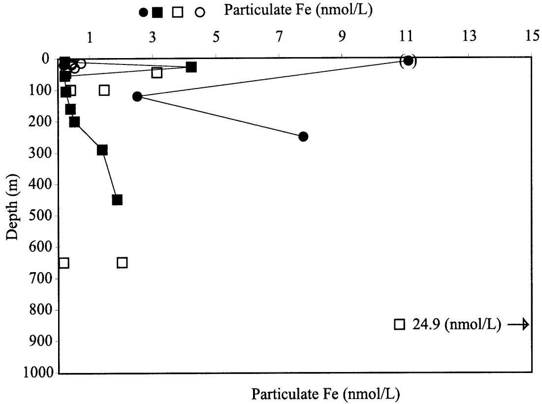
Figure 5.10 Particulate Fe samples from the Eastern Tropical Pacific profile (black squares), BATS profile (black circles), California Borderland Basin samples (open squares) and the Sargasso Sea surface samples (open circles). Arrow indicates deep sample from near the bottom of the San Nicholas Basin, the high value is likely due to sediment resuspension. Bracketed samples indicate surface samples that may have been contaminated during collection.
