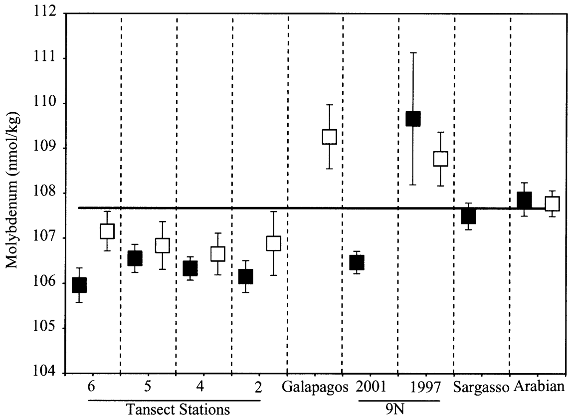
Figure 3.10 Chart of average salinity normalized concentrations separating filtered (filled squares) and unfiltered (open squares) data sets. Error bars represent 2 times the standard error. The solid line represents the average Mo concentration of seawater. The Arabian Sea and Sargasso profiles are equivalent to the average seawater value. The 16N transect and the 9N 2001 profiles are all depleted throughout, while the 9N 1997 and Galapagos profiles are enriched. Unfiltered samples tend to have larger variability than the filtered samples, perhaps due to particle contributions.
