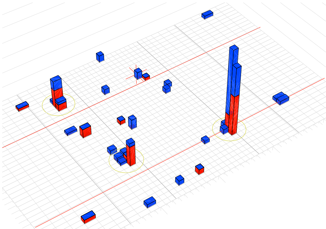
Figure 3. \eta - \phi view. Top pictures shows a 2D option of the view, where cell size represent energy and color corresponds to the calorimeter that made the biggest contribution. Bottom picture shows a standard 3D Lego option.
