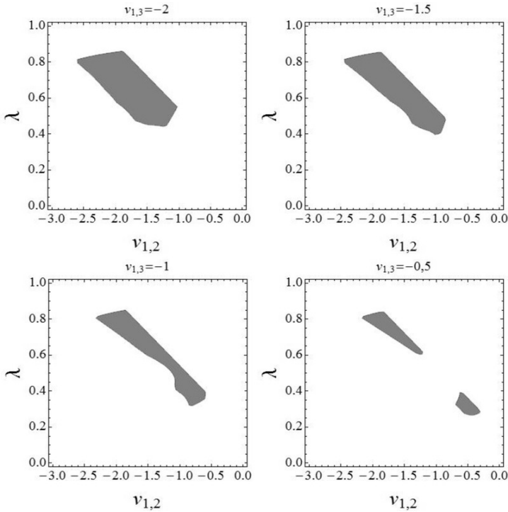
Figure 2. A- and L-stable methods of stage order q = 5 and order p = 6
