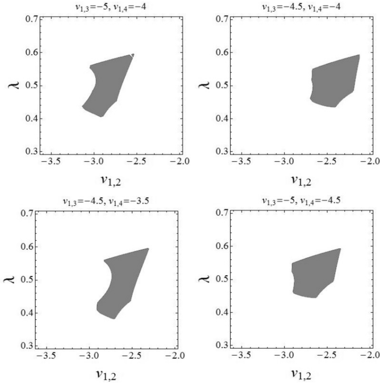
Figure 3. A - and L -stable methods of stage order q = 6 and order p = 7 .
