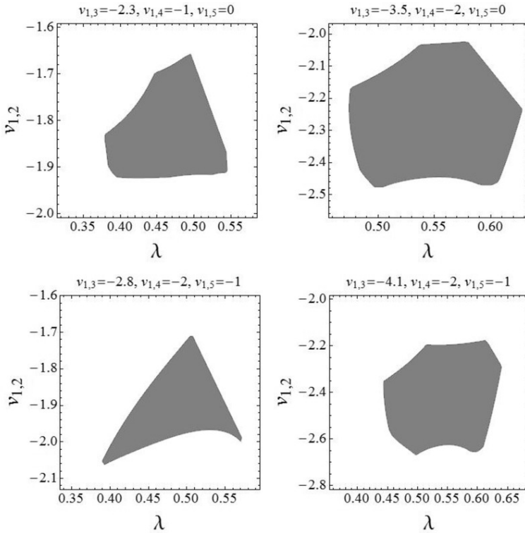
Figure 4. A - and L -stable methods of stage order q = 7 and order p = 8 .
