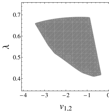
Figure 1. A - and L -stable methods of stage order q = 4 and order p = 5 .
