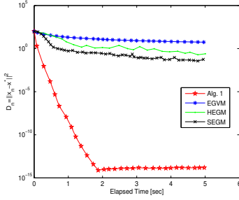
Figure 1. Experiment in \mathbb{R}^{100} for \alpha_n = \frac{1}{\sqrt{n+1}}
