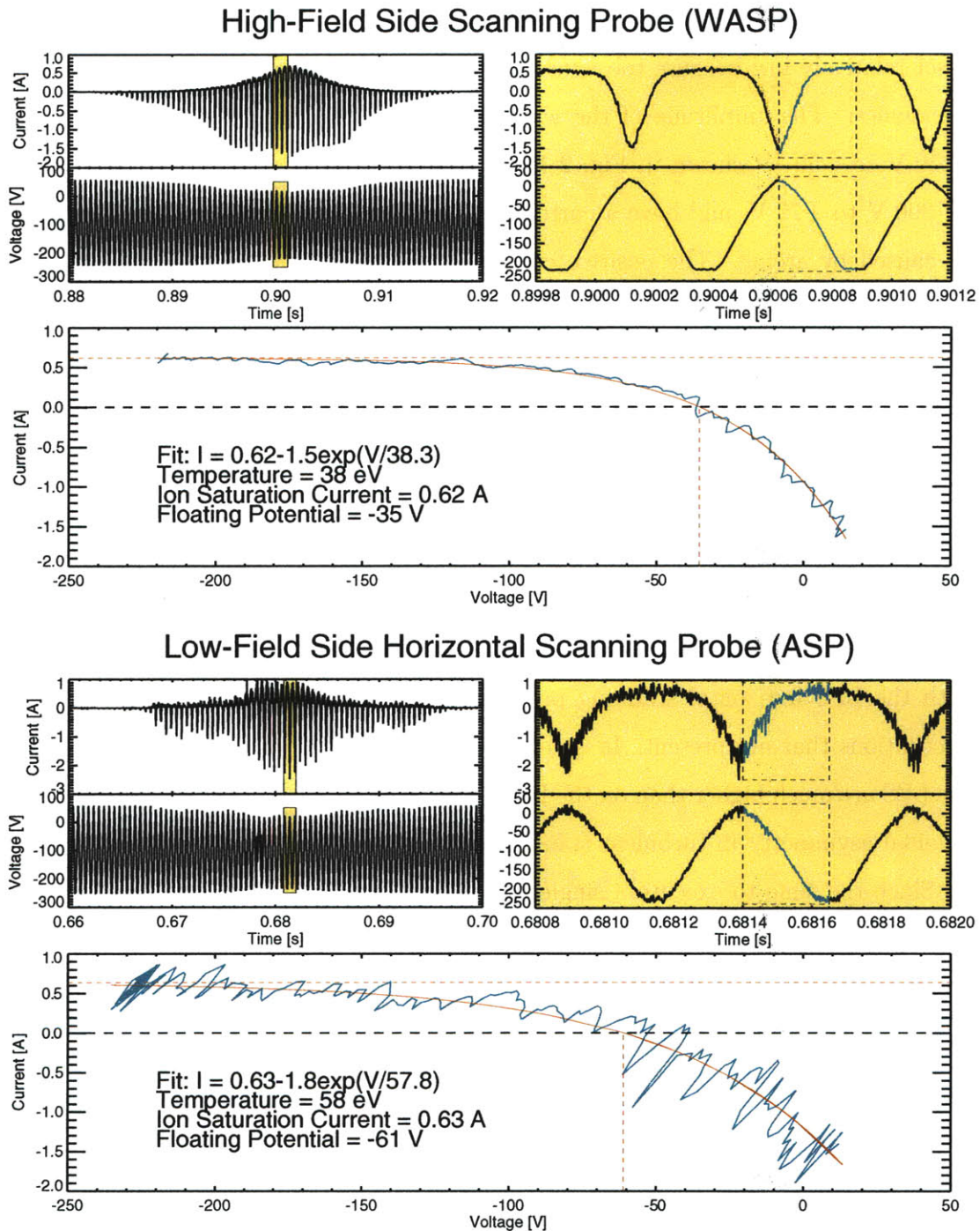
Figure 2-14: This figure shows time traces of the current and voltage on a scanning probe as a function of time during a single probe plunge. A roughly triangular voltage waveform with a frequency of 2 kHz is applied to the electrode. The upward and downward going I - V sweeps are each fit with an exponential to provide 4 kHz measurements of electron temperature, density and floating potential. Examples are shown for a WASP and ASP I - V fit. Note the smaller fluctuation levels in the high-field side data.
