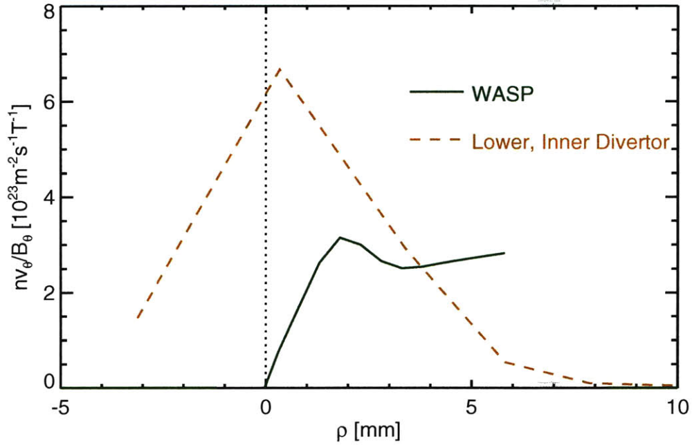
Figure 8-23: nv_{\theta}/B_{\theta} is the particle flux density normalized to the poloidal magnetic field. This quantity is constant flux surface for divergence-free flows. This allows us to compare flux densities measured at different poloidal locations. Here, we see that the particle flux density passing the WASP in the near SOL is much less than that arriving at the divertor, indicating a high-recycling state. In the far SOL, it is the opposite, with much higher flux densities at the WASP than the inner divertor. This is consistent with a region of volume recombination in the far SOL.
