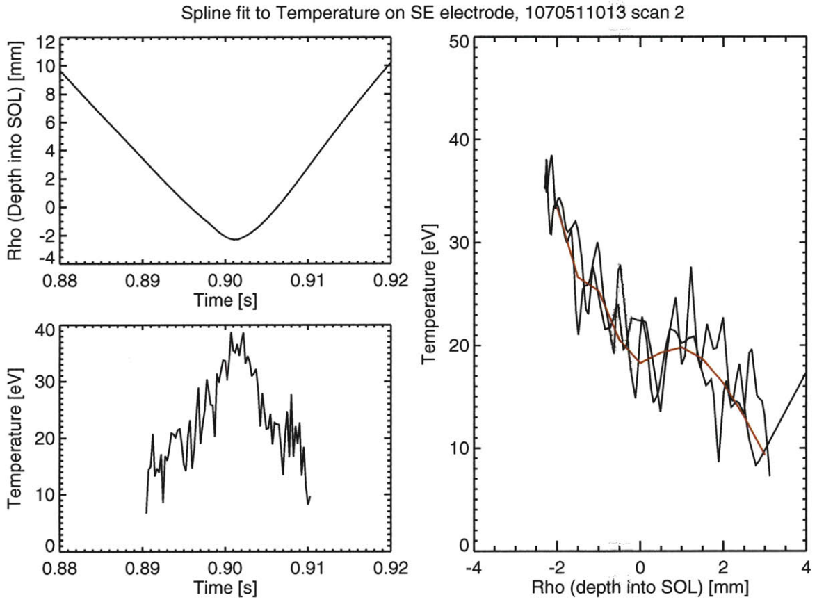
Figure 2-15: An example of a mapping of the temperature measurement on a single electrode during a single probe plunge from time space into \rho -space. The ingoing and outgoing traces overlay well, as is typically the case. The spline fit to the data is shown. The data in the remainder of the thesis will be presented in this format.
