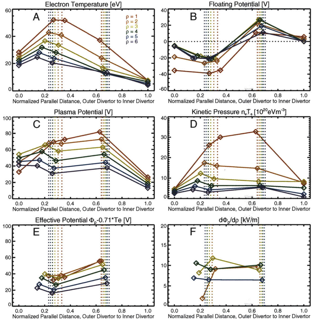
Figure 4-5: Plasma potential and related data are shown as a function of normalized parallel distance from outer divertor to inner divertor. The five points on each trace are the locations of the probe diagnostics in this space. From left to right these are the outer divertor embedded probes, the F-port vertical scanning probe, the A-port horizontal scanning probe, the wall scanning probe and the inner divertor embedded probes. The different color traces are data from different locations in \rho -space, red being very close to the LCFS and purple being 6 mm deep into the SOL. The dashed vertical lines show the locations of the LFS and HFS midplanes for each \rho location plotted.
