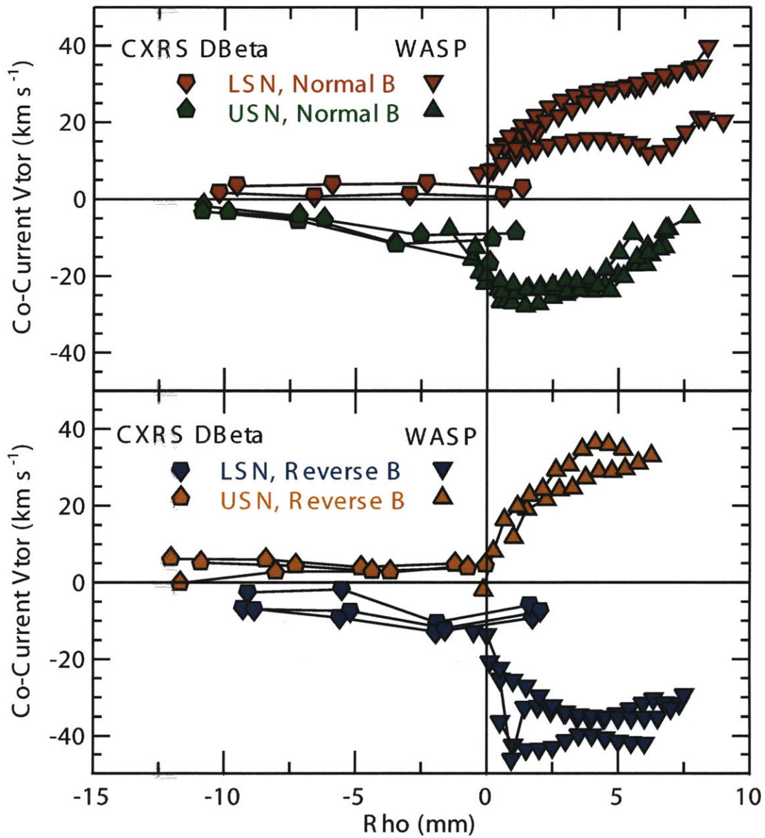
Figure 7-6: A comparison of the parallel velocity measured by the WASP to that measured with the HFS main-ion ( D\text{-}\beta ) charge exchange system for a selection of typical discharges. Based on the sign convention (co-current parallel flows = positive), the positive direction changes with field/current reversal. Thus, the two cases with favorable drift direction (red and orange) can be directly compared, as can the cases with unfavorable drift direction (green and blue).
