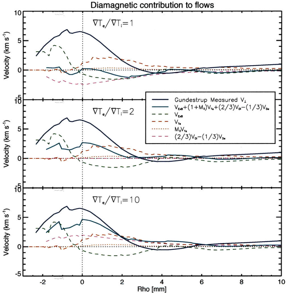
Figure 5-7: A comparison of Hutchinson's model for Gundestrup perpendicular flow measurements with the experimental results. The three panels show the Gundestrup V_{\perp} measurement along with Hutchinson's prediction for different assumptions about the ion temperature gradient. The different terms of Hutchinson's formula are also shown. The data are from the ASP during medium density discharges ( 1.04 < \bar{n}_e < 1.52 [10^{20} \text{ m}^{-3}] ) on the 1070627 run day.
