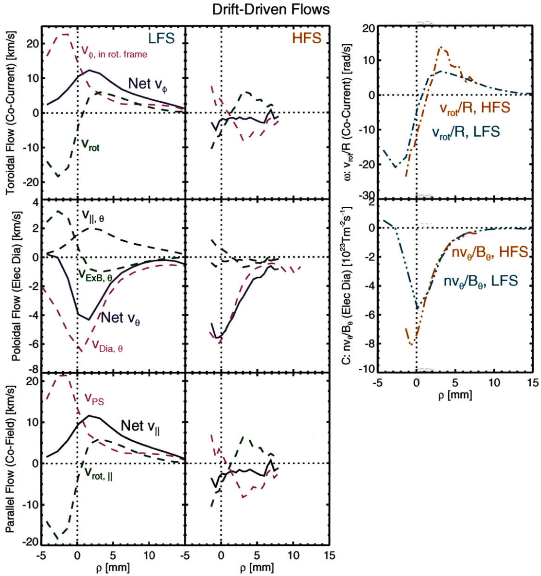
Figure 8-5: The toroidal and poloidal components of the drift-driven flows from Fig. 8-2 are shown in the top two rows of plots. The components are determined according to the vector manipulations illustrated in Fig. 8-4. The first column shows the LFS location and the second column shows the HFS location. The third column shows the constants \omega and C at these two locations. Both are observed to be independent of poloidal location, as expected for a divergence-free flow with potential and pressure constant on a flux surface. The third row shows the components of measured parallel flow.
