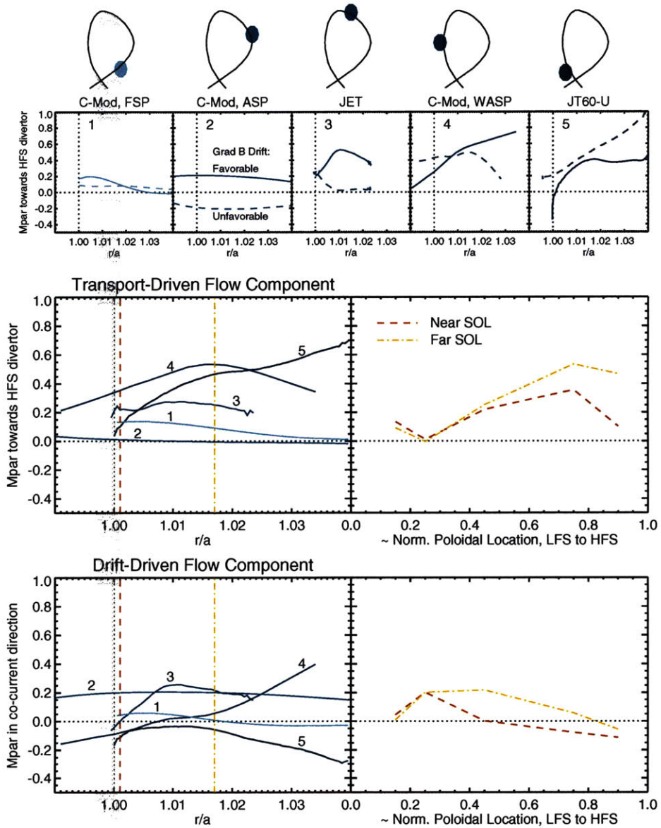
Figure 7-4: A comparison of parallel flows measured on Alcator C-Mod, JET and JT60-U at a variety of poloidal locations. The top panels show the measurements from each location for forward and reversed field. The second row, left-hand panel shows measurements from each location averaged for favorable and unfavorable drift direction, or ‘transport-driven flow component’. The right-hand panel shows this flow component as a function of poloidal distance at the r/a locations indicated in the left-hand panel. The last row shows half the difference between the favorable and unfavorable parallel flow measurements, or the ‘drift-driven flow component’.
