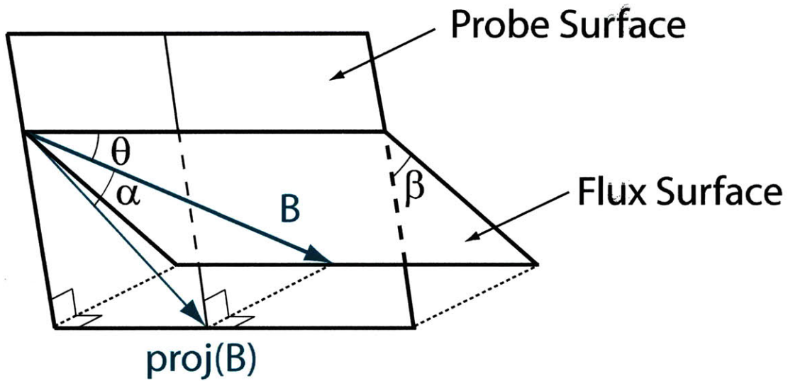
Figure 5-2: An illustration of the various angles discussed in this section. The angle \beta is the angle between the flux surface and the probe surface. This is equivalent to the ‘pyramid steepness’ and is 45^\circ on the C-Mod high-heat flux Gundestrup probes. For most previous Gundestrup experiments, this angle has been 90^\circ . The angle \theta between the field and the probe surface within a flux surface is the primary quantity used in the Gundestrup formulation. On the C-Mod probes, this angle is also \sim 45^\circ . The angle \alpha is the simple angle between the field and the surface, that is, the angle between the field and its projection onto the surface. For probes with \beta = 90^\circ , \alpha = \theta . On C-Mod, \alpha \approx 30^\circ .
