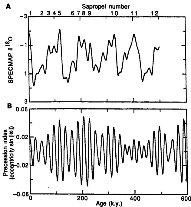
Figure 5.6: Stratigraphic position of Late Quaternary Eastern Mediterranean sapropels within (a) the SPECMAP stacked \delta^{18}\text{O} record of Imbrie, et al (1984), and (b) the orbital precession index of Berger and Loutre (1991). Sapropels S2 through S7 were included in this study. Figure from Emeis, et al (1996).
