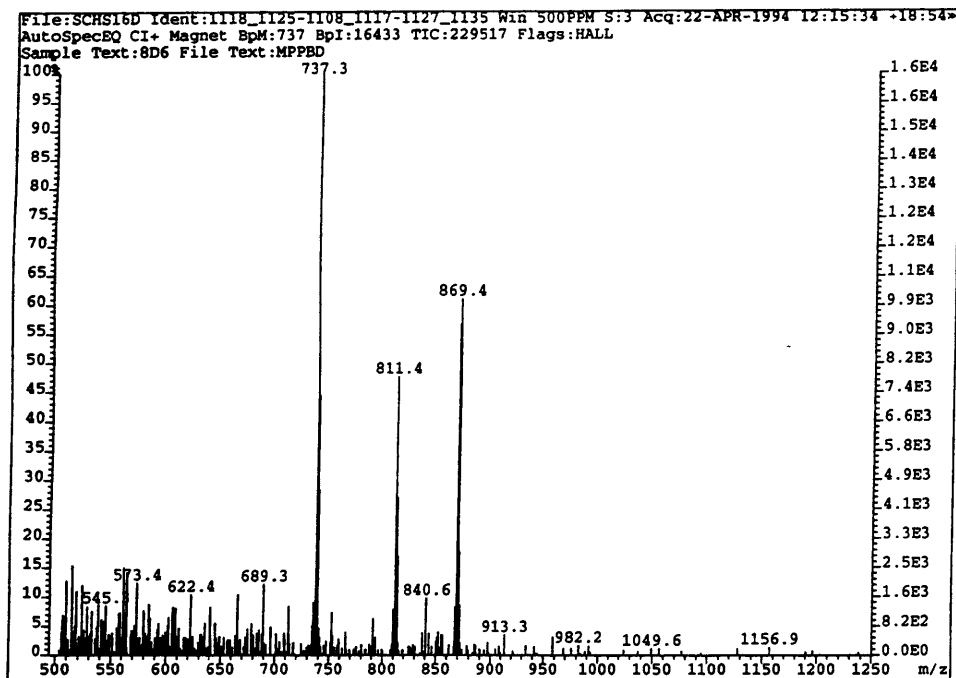
Figure 3.21: GC-Cl + mass spectrum of compound eluting 19 seconds after (MPPBDa)Si(OTBDMS) 2 . The fragmentation pattern is virtually identical to that of the desired product (figure 3.20), yet each fragment is 32 mass units greater (see text for discussion).
