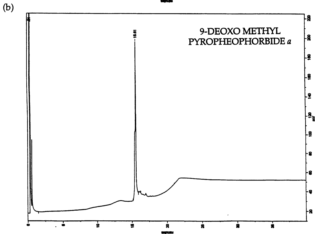
Figure 3.24: Gas chromatograms of (a) deuterioporphyrin IX dimethyl ester, and (b) 9-deoxo-methyl pyropheophorbide a .
