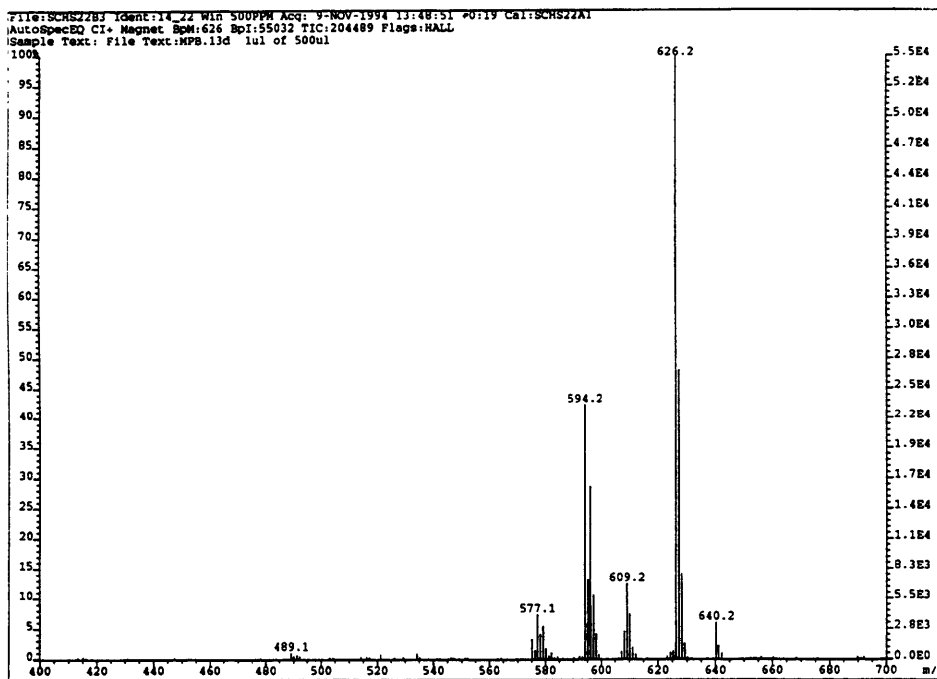
Figure 3.7: Methane chemical ionization mass spectrum of (9MPPBDa)Si(OH) 2 (M/Z = 594 (M, 40%)). In addition, a product with M/Z = 626 was formed (M+32, 100%), which corresponds to the addition of CH 4 O. A discussion of this product can be found in section 3.6.4.
