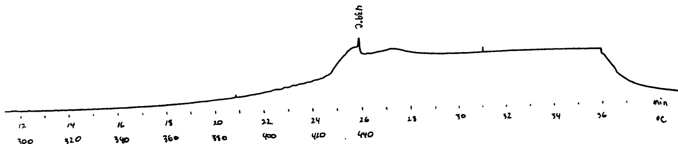
Figure 3.23: Gas chromatogram of methyl pyropheophorbide a . Partial thermal decomposition of the chlorin occurred prior to its elution at 439°C.
