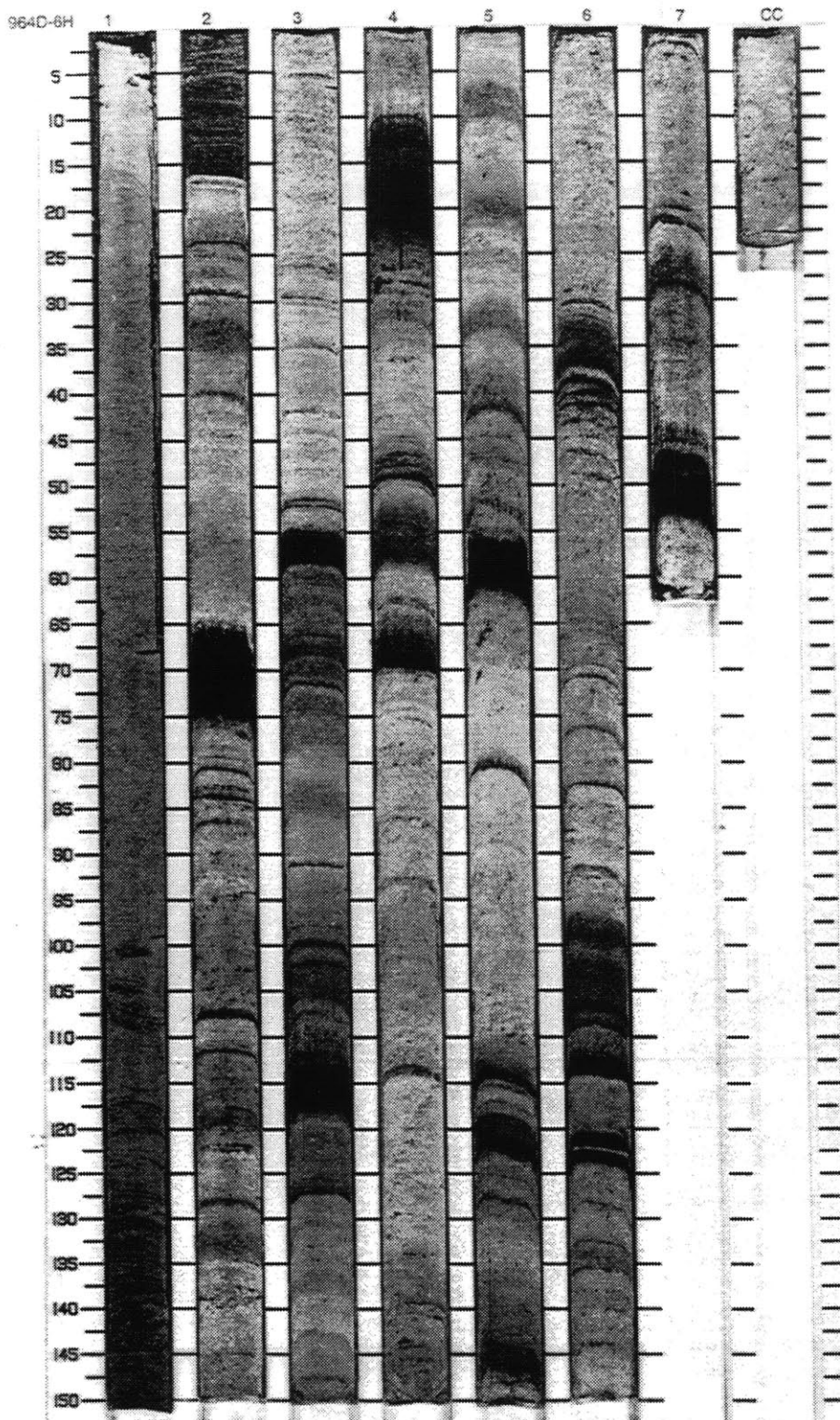
Figure 1.4: Typical example of sapropels recovered from the Eastern Mediterranean. Sapropels are the dark bands.
