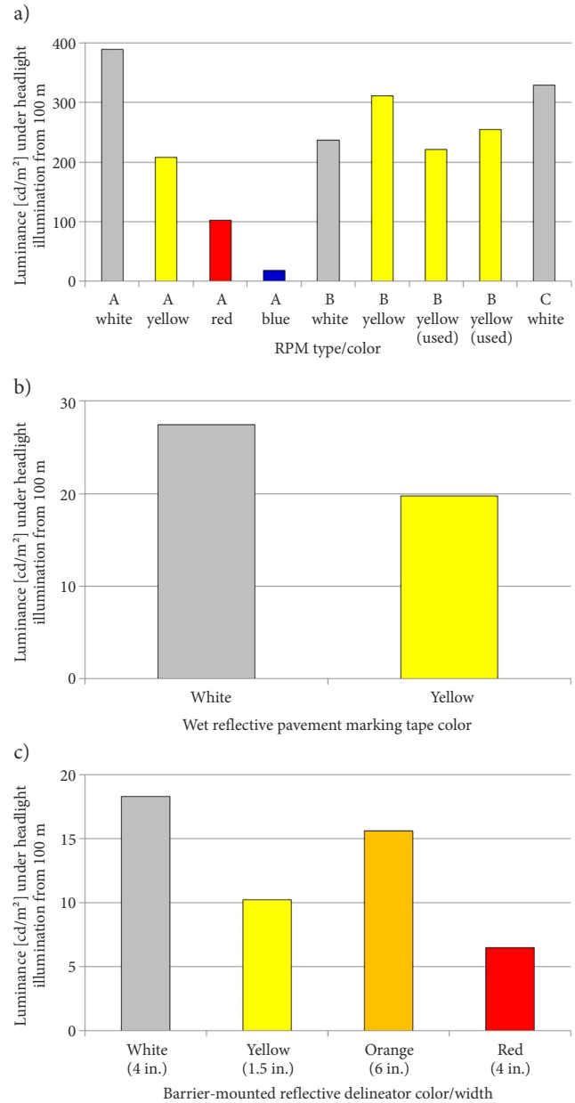
Figure 8. Luminances [cd/m 2 ] under headlight illumination from 100 m away for: a – RPMs; b – wet reflective pavement marking tape; c – barrier-mounted reflective delineators
