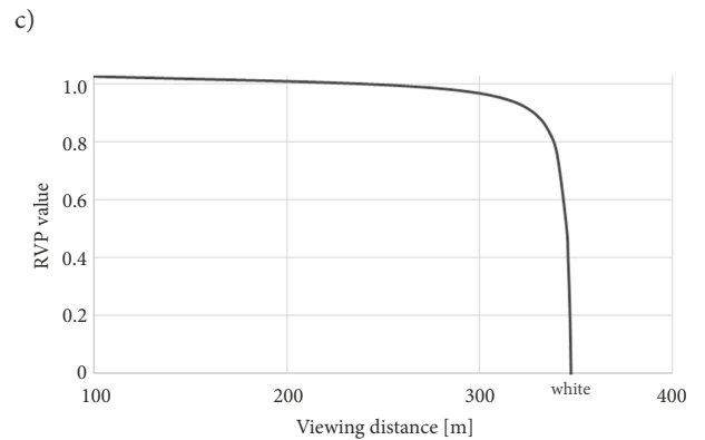
Figure 10. RVP values for each RPM type and color, as a function of viewing distance: a – Manufacturer A; b – Manufacturer B; c – Manufacturer C
