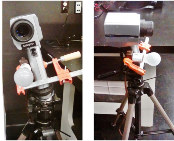
Figure 4. Luminance meter and light source (left: front view, right: side view)
