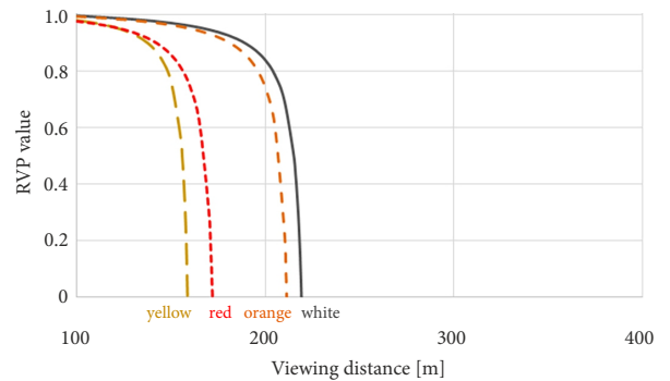
Figure 12. RVP values for each barrier-mounted reflective delineator color, as a function of viewing distance
