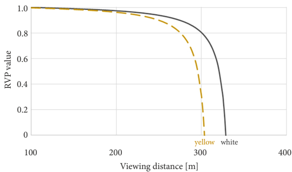
Figure 11. RVP values for each wet reflective pavement marking tape color, as a function of viewing distance
