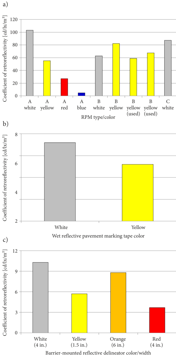
Figure 7. Coefficients of retroreflectivity [cd/lx/m 2 ] for: a – RPMs; b – wet reflective pavement marking tape; c – barrier-mounted reflective delineators
