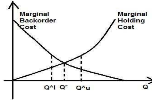
Figure 5-2: Decision of Order Size
