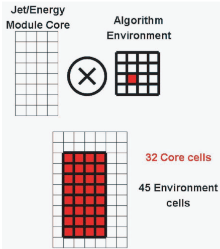
Figure 5: Core and environment jet elements considered by an individual Jet/Energy sum Processor module.
