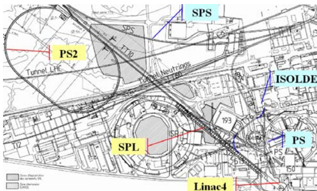
Figure 1: Layout of the new injector complex.
