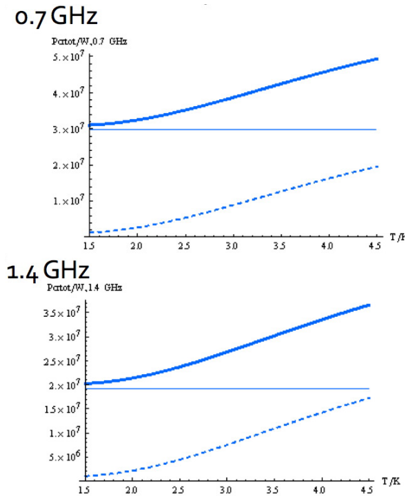
Figure 3: Electric power consumption as a function of temperature (arbitrary units). The curves show the cryogenic power, RF power, and the sum (bottom to top).
