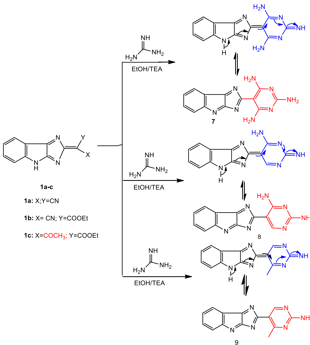
Scheme 4. Synthetic routes for the compounds 7-9.
