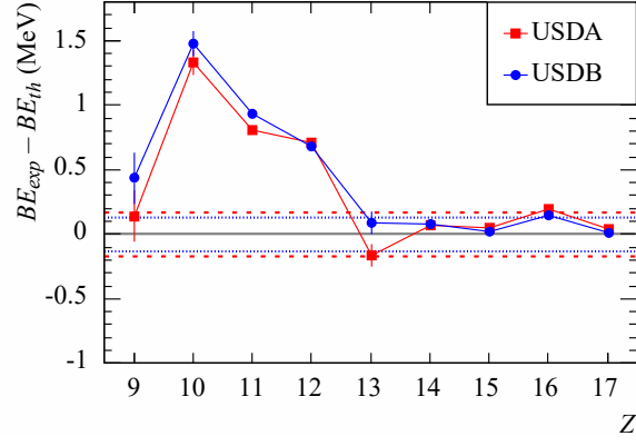
FIG. 4. (Color online) Difference between experimental and theoretical (USDA, USDB) binding energies for N = 19 isotones, 9 \leq Z \leq 17 . The error bars on the data points represent experimental errors only. The blue dotted, red dashed, and black dash-dotted bands represent the respective 170 and 130 keV RMS deviations of USDA and USDB interactions. Experimental values, save for Z = 9 which is from the present work, are taken from [16] if reported there; otherwise they are from the 2003 Atomic Mass Evaluation [34].
