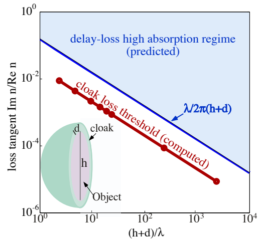
FIG. 2: Maximum cloak loss tangent versus diameter h for cloaking a perfectly conducting sphere, for cloak of thickness d = h/12 . Shaded area is the regime of high absorption predicted by the simple 1d model of Eq. (2). The red curve, data from Ref. 12, shows the maximum loss tangent to obtain 99% reduction in the scattering cross section using a Pendry-type cloak.
