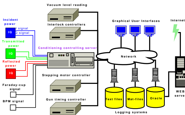
Figure 3: The computer architecture.
