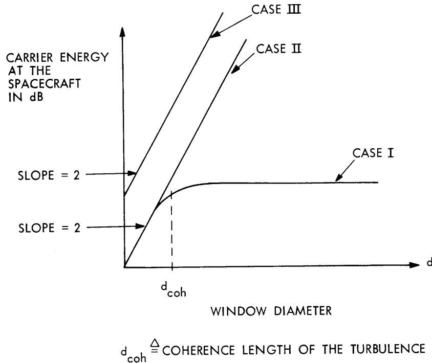
Fig. XXII-3. Performance comparison.
