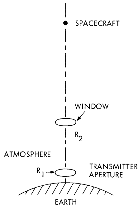
Fig. XXII-1. Apodization problem.
