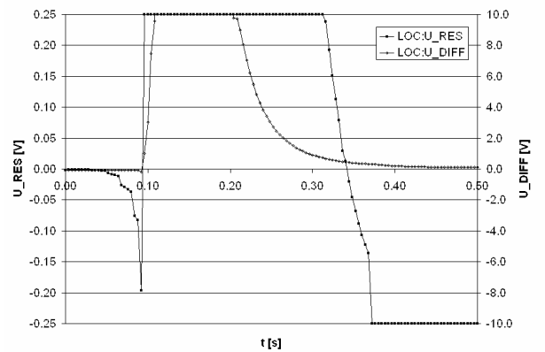
Figure 2: Natural quench observed in the RCD.A56B1 corrector magnet circuit at I = 535 A during first powering to nominal current ( I = 550 A). The circuit comprises 77 decapole spool piece correctors type MCD. The calculated resistive voltage U_{RES} and the measured voltage U_{DIFF} saturate respectively at \pm 0.25 V and \pm 10 V.
