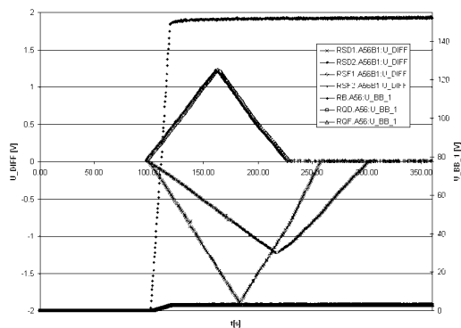
Figure 4: Ramping of multiple circuits. The graph shows the differential voltages across the superconducting part of the main dipole and quadrupole circuits as well as a selection of lattice sextupole circuits.
