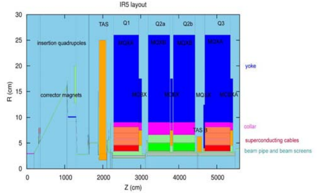
Figure 4: IR5 layout
