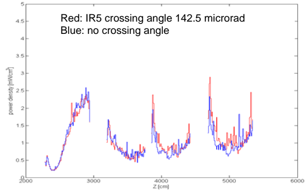
Figure 7: Longitudinal distribution of peak power density in the inner cable for Q1 and Q3 ( 3.5 < R < 4.6 cm) and for Q2a and Q2b ( 3.5 < R < 5 cm), effect of the crossing angle.
