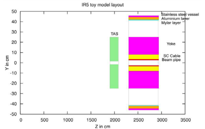
Figure 1: Layout for the comparison
