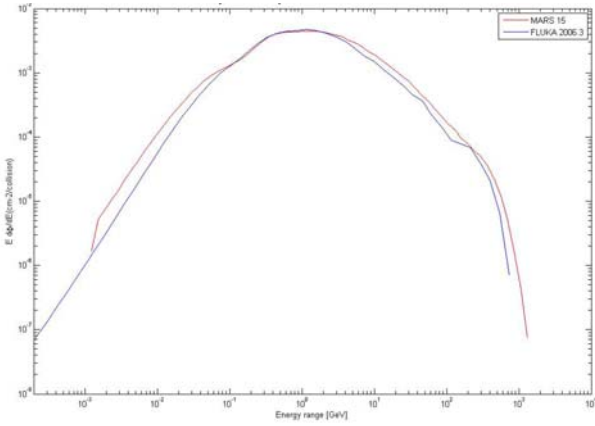
Figure 3: Pion & kaon spectra in cable1
