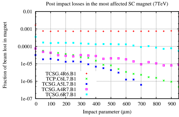
Figure 4: Fraction of the beam lost in the most affected superconducting magnet after an initial impact in different collimators as a function of the impact parameter.
