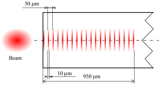
Figure 2: Configuration of the initial distributions of particles generated before each collimator. The collimator representation does not correspond to the collimator real shape and is not to scale.
