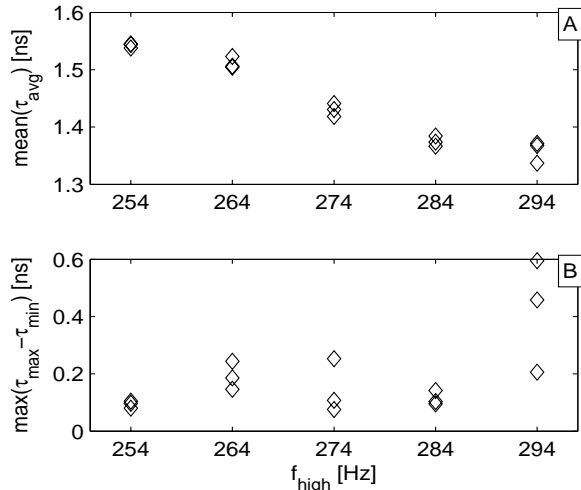
Figure 3: Average bunch length (A) and maximum oscillation across the batch at the FT (B), each point a different MR, plotted versus noise high cutoff frequency ( f_{\text{high}} ). All with A_n = 400 mV and \phi_{\text{offset}} = 223^\circ .
