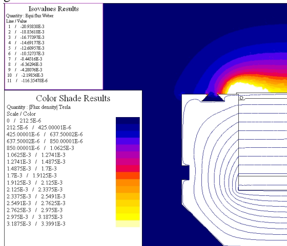
Figure 3: BISMV cross section showing the 1% (stray) field region.
