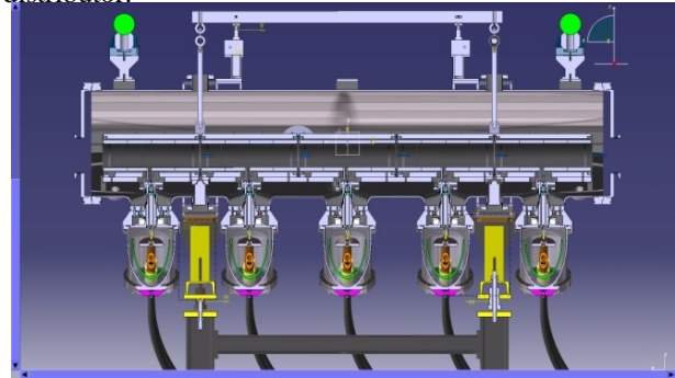
Figure 2: BIDIS assembly cross section, showing the 5 magnets inside the vacuum vessel and the associated feedthroughs and connection boxes below the tank.
