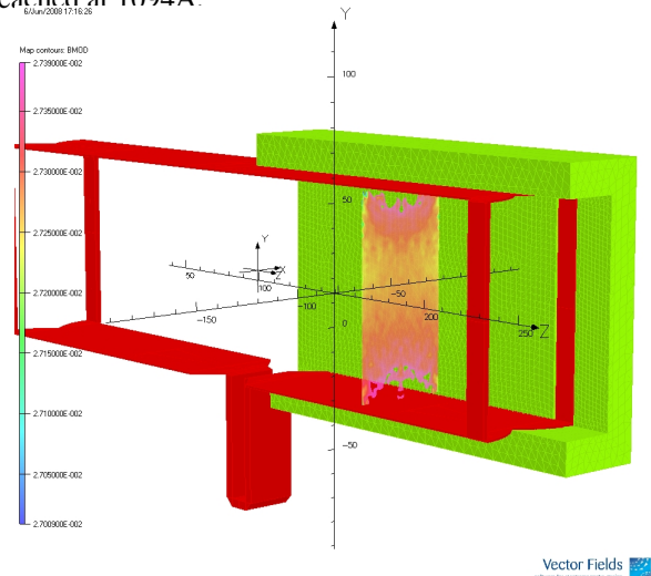
Figure 1: Finite element model of BIDIS with the 1 % field region plotted.
