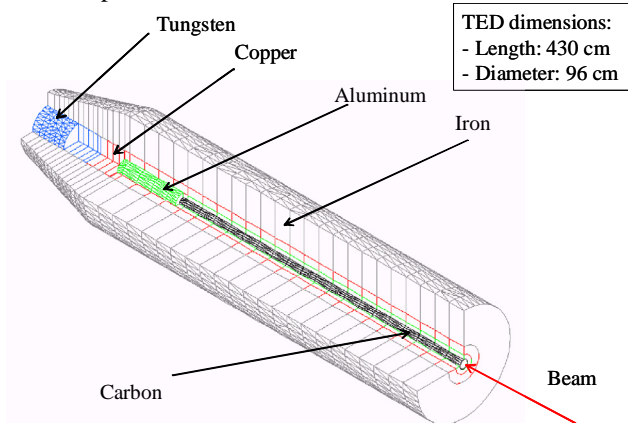
Figure 2. Geometry of SPS dump used for simulation.
