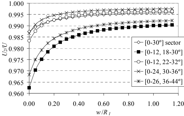
Figure 2 - Ratio between the magnetic energy produced by the main harmonic ( n=2 ) and the total energy versus w/R_1 for five different sector coils.
