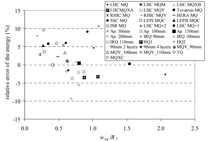
Figure 3 - Agreement between numerical estimate of magnetic energy and analytical estimate for a 30° sector coil based on (10).
