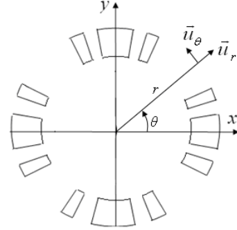
Figure 1 - Cross-section of a Quadrupole magnet made of 2 pure sectors.
