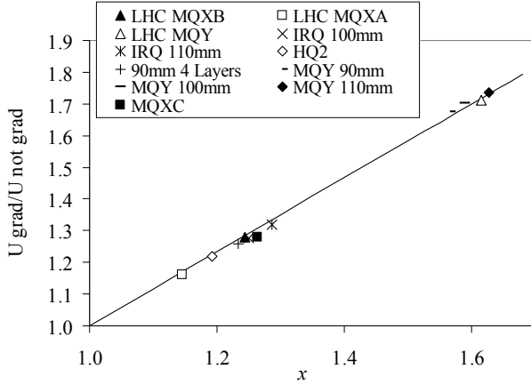
Figure 4 - Increase of magnetic energy due to grading as a function of x as defined in (16).
