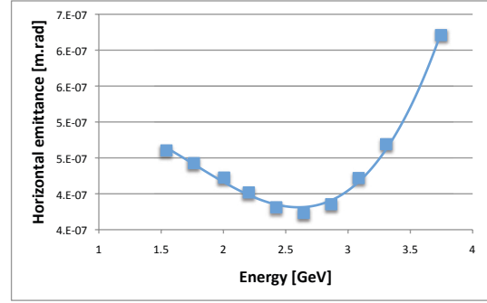
Figure 4: Horizontal emittance dependence on the energy while keeping a constant longitudinal emittance.
