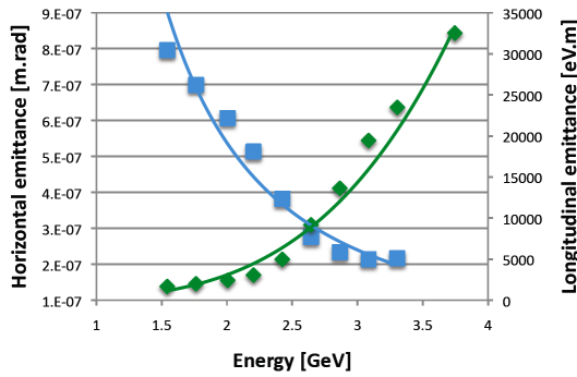
Figure 3: Horizontal (blue) and longitudinal (green) emittance dependence on the energy.
