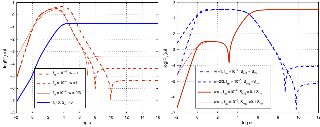
FIG. 2 (color online). The evolutions of \Psi_k (plot at the left) and of \mathcal{R}_k (plot at the right) are illustrated. In the right plot the cases \mathcal{S}_{mS} = \mathcal{S}_{mr} and \mathcal{S}_{mS} \ll \mathcal{S}_{mr} are compared.
