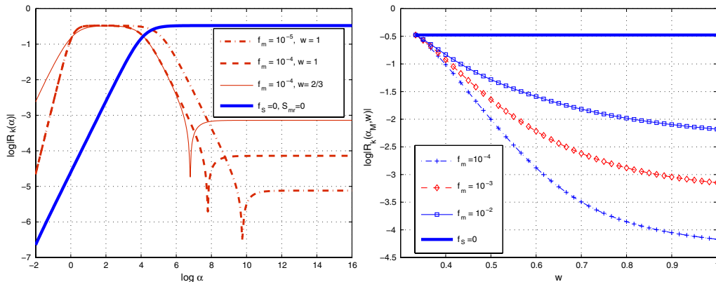
FIG. 1 (color online). The evolution of the curvature perturbations as a function of the scale factor and for various fixed values of w (plot at the left); the evolution of curvature perturbations for fixed \alpha \gg 1 and as a function of the sound speed of the stiff component (plot at the right).
