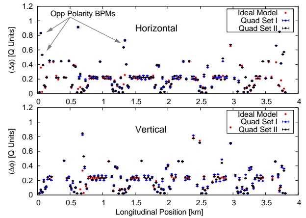
Figure 4: Measured phase advance between RHIC BPMs after trimming 1 st set of three quadrupoles (blue) and the 2 nd set (black) compared to the ideal model (red). Vertical error bars are statistical deviation between three consecutive data sets with the same condition
