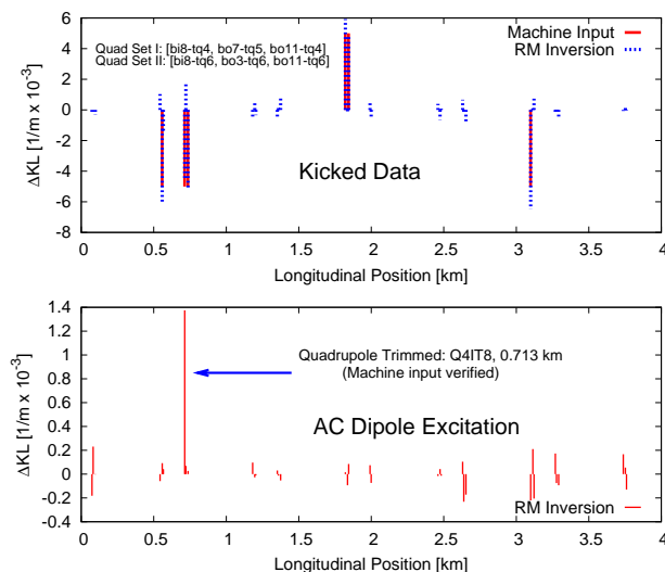
Figure 6: Top: Quadrupole trims predicted by RM inversion onto the measured phase beat from kicked data compared to the input trims into the machine. Bottom: Quadrupole trim predicted by RM inversion onto measured phase beat using an ac dipole excitation.
