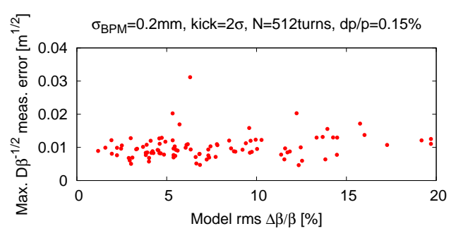
Figure 3: Maximum error in ND measurement vs. rms \beta -beating (simulation) for a 100 of LHC machines with errors.
