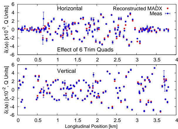
Figure 5: Measured phase beat between RHIC BPMs after trimming six quadrupoles by \pm 0.005 \text{ m}^{-1} randomly.
