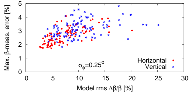
Figure 1: Maximum error in arc \beta measurement vs. r.m.s. model beta-beating. Phase error is assumed \sigma_\phi = 0.25^\circ .
