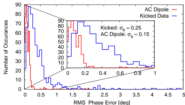
Figure 7: Histogram of the rms phase noise from the all the BPMs from several data sets both from kicked data and ac dipole excited data.
