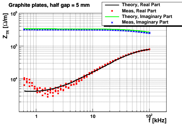
Figure 3: Real and imaginary part of the transverse impedance of graphite plates (stage 1 in Table 1).
