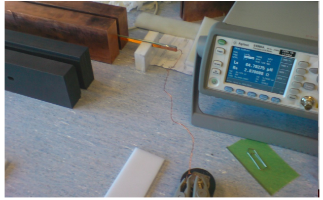
Figure 2: Experimental setup example: LCR meter, graphite and copper jaws, probe coil inside the copper jaws.
