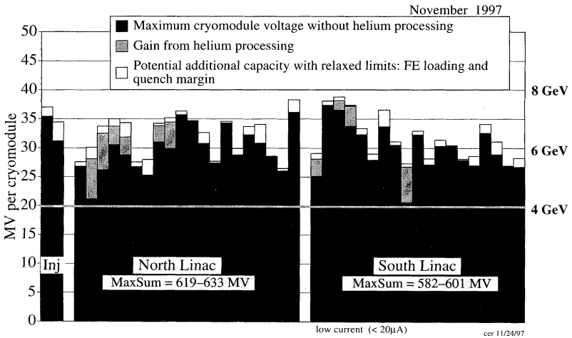
FIGURE 3 Maximum voltages obtainable from the CEBAF cryomodules.
