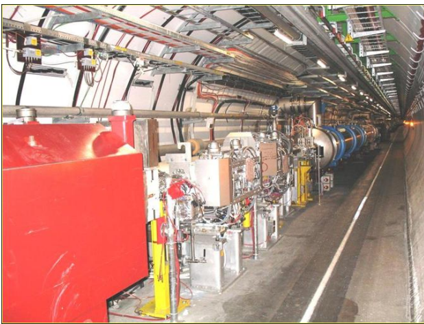
Figure 4: Beam instrumentation, collimators and other equipment presently installed in between the TAN (red object on the left) and the D2 separation dipole (blue cryostat on the right) in the ATLAS matching section.
