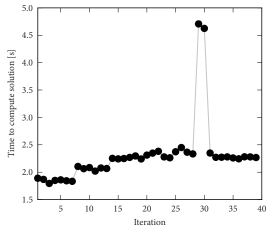
Figure 6. Time taken per iteration: real-time testing
