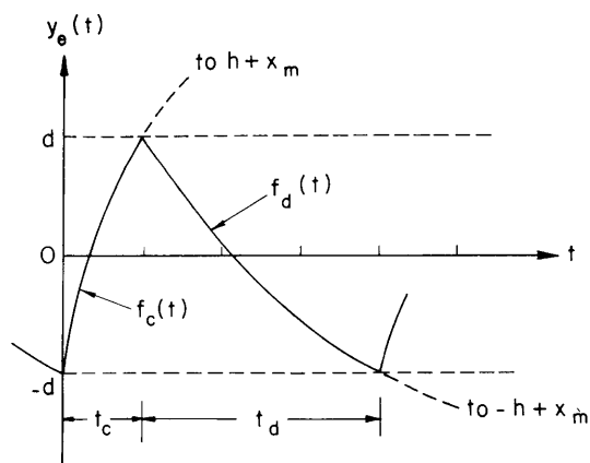
Fig. XXV-3. Exponential-error waveform.
