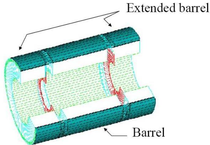
Figure 1: Tile Calorimeter.
