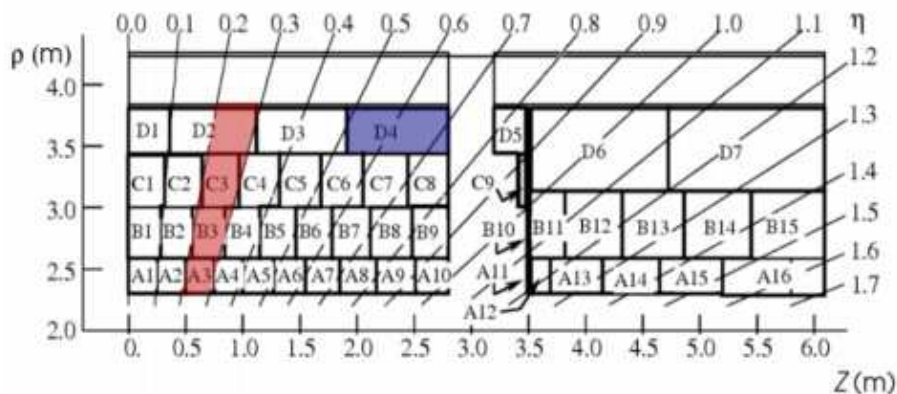
Figure 2: Tile Calorimeter segmentation.
