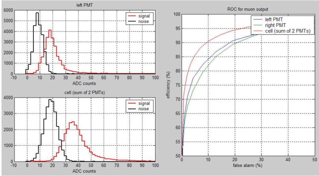
Figure 4: Peak detector efficiency.
