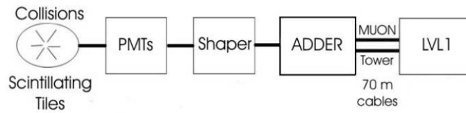
Figure 3: Readout from Tile Calorimeter.
