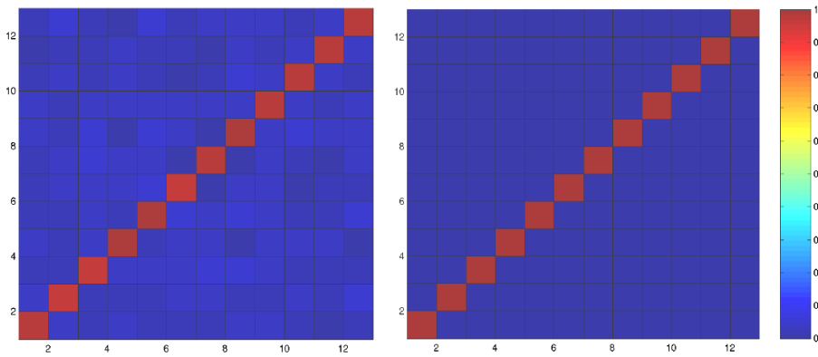
Figure 6: Covariance matrices of the test and development set.
