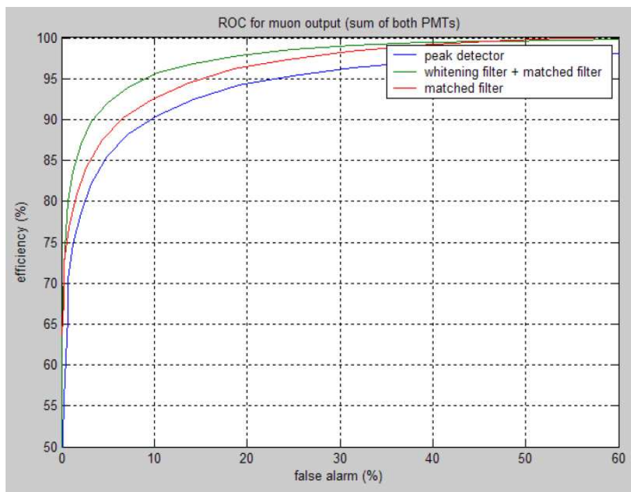
Figure 7: Comparison between peak detector and matched filter (with and without whitening filter).
