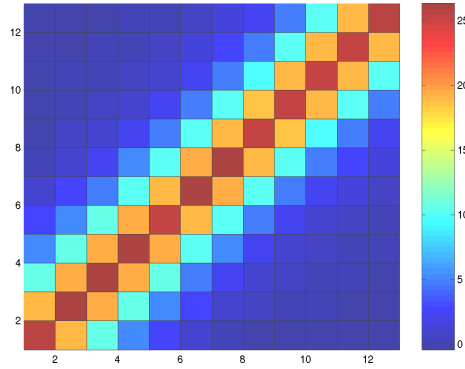
Figure 5: Covariance matrix of the development set.
