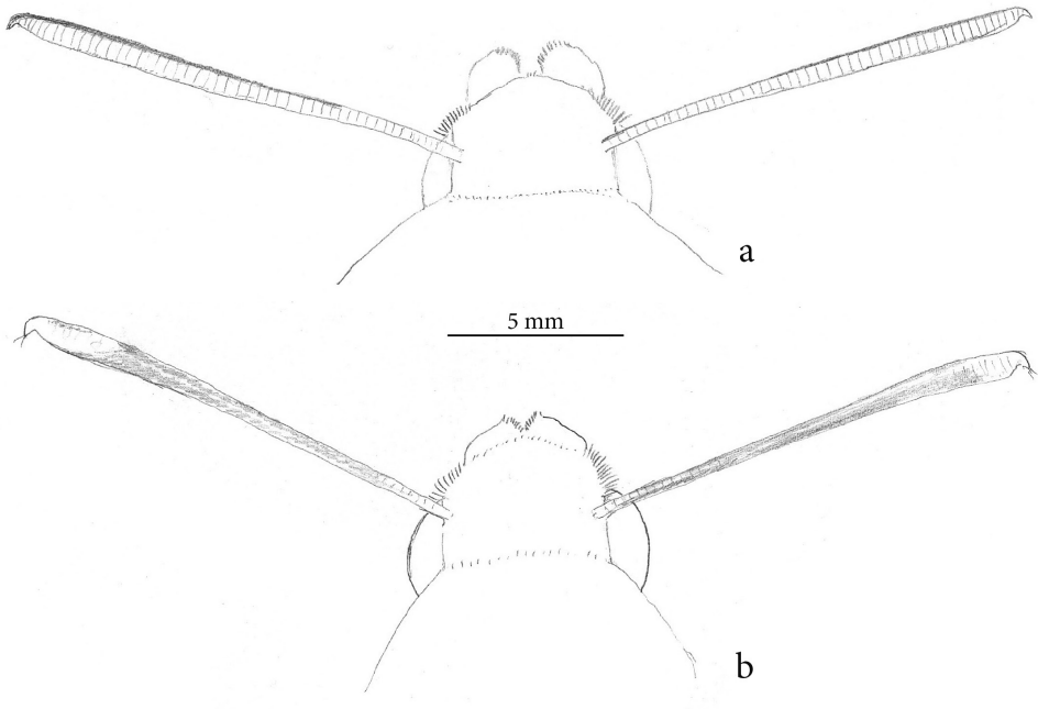
Figure 1. Head (dorsal view) of (a) Hyles euphorbiae (Germany, Dresden, coll. Barkowski, MTD, same individual as Fig. 9c) and (b) H. livornica (Italy, Cuma-Campania, dune area, leg. R. Remane, MTD, same individual as Figs 5c, 6f, 9b).
