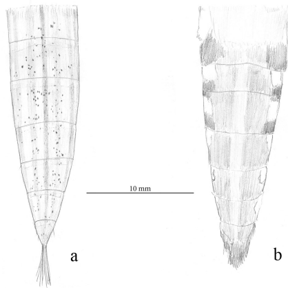
Figure 7. Abdomen segments 2–8 of (a) Xylophanes loelia (Druce, 1878) (Brazil?, Para, leg. S. Wähler, MTD), (b) Hyles euphorbiarum (Chile, MTD).
