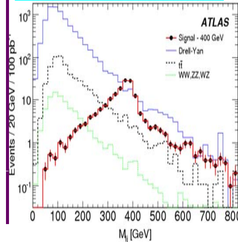
After basic selection but before background suppression
