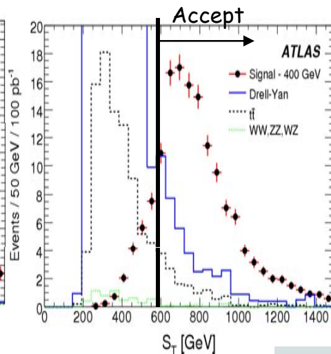
S_T :pT scalar sum
