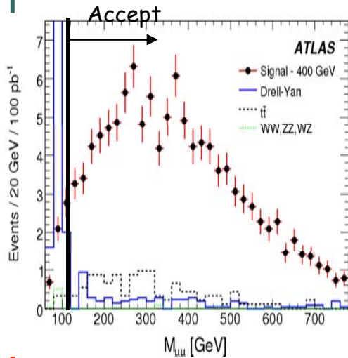
Dilepton invariant mass
