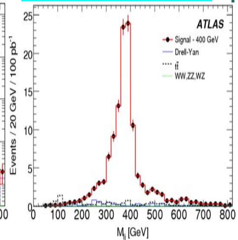
After basic selection and after background suppression
