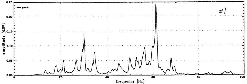
FIGURE 2: Typical spectrum of phase error signal
