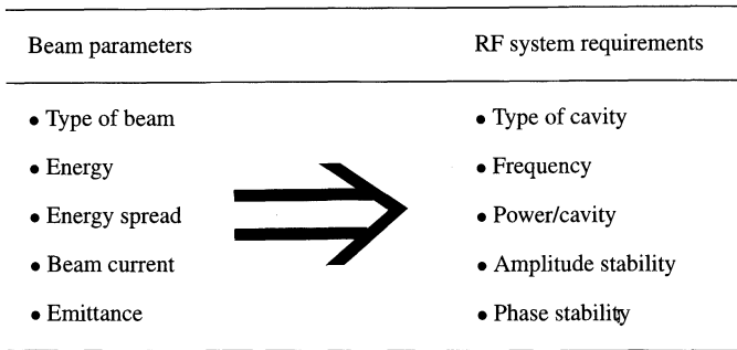
FIGURE 1: RF system parameters are driven by beam parameters.
