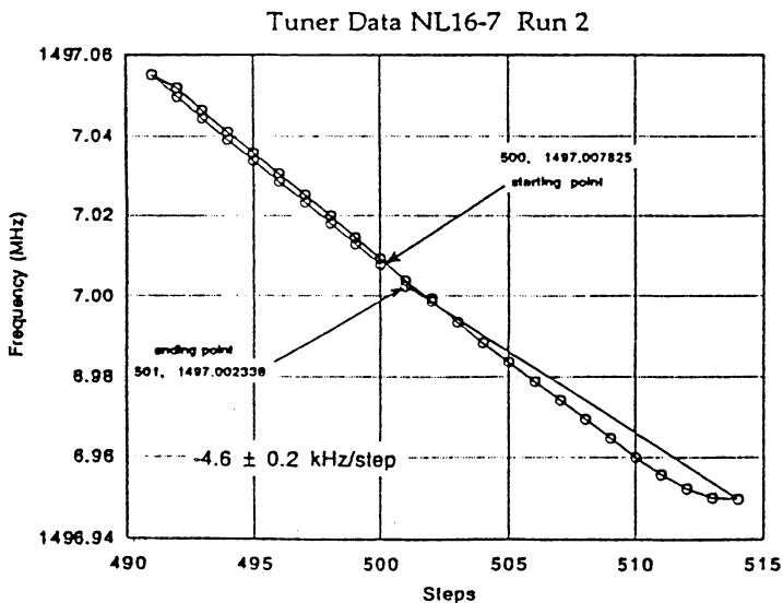
FIGURE 4: Typical tuner hysteresis
