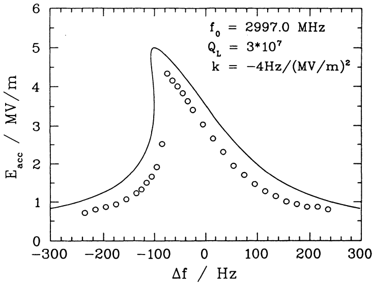
FIGURE 2: Influence of radiation pressure on the resonance of a sc cavity. Open circles represent a measurement on one of the S-DALINAC cavities.
