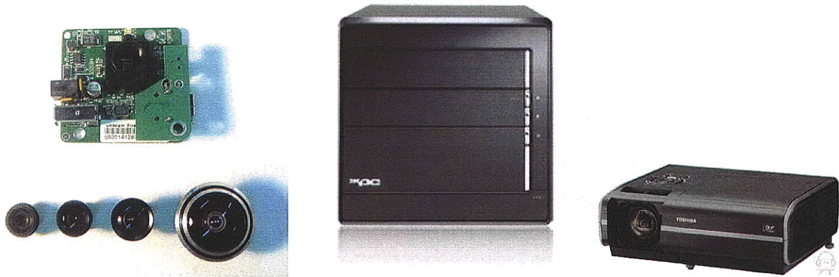
Figure 67. Hardware: Fire-I Camera and lens, Shuttle PC 3600, and Toshiba EX20 Short Throw Projector
