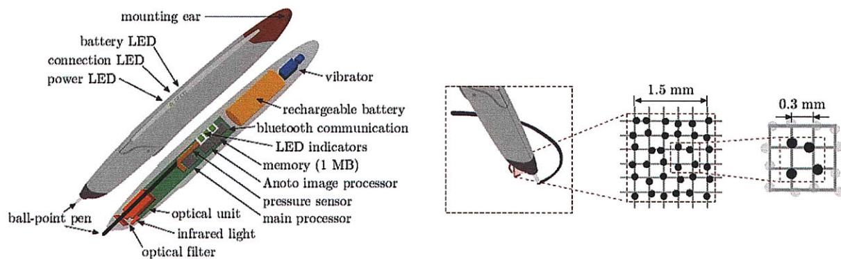
Figures 70b, 70c. Schematic of Anoto components and Anoto Pattern. Courtesy of Jacob Leitner, MIL, 2008
