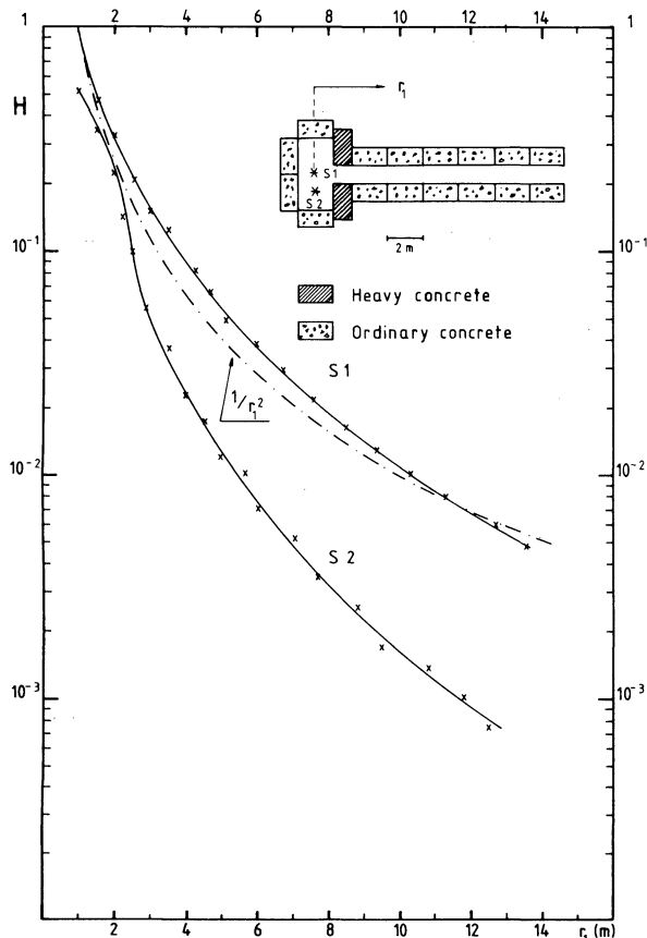
FIGURE 1 Dose equivalent attenuation in a straight access way. Two source positions S_1 and S_2 are indicated.
