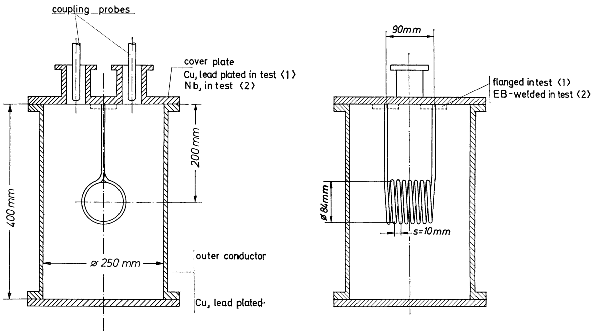
FIG. 2. Cross section of the helically-loaded resonator.
