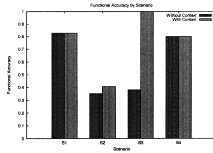
(b) Functional Accuracy by Scenario
