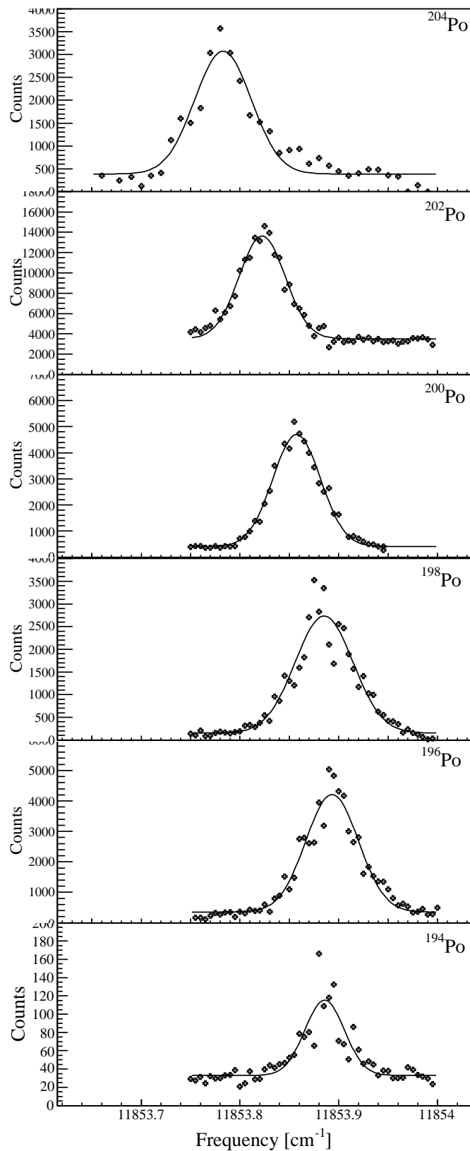
Figure 2: Optical spectra for the even- A isotopes ^{194},^{196},^{198},^{200},^{202},^{204}\text{Po} . The fitted line is a simple Gaussian profile; a detailed analysis taking into account the total line shape is ongoing.
